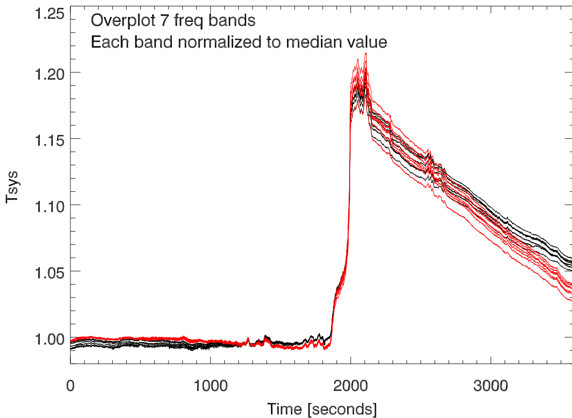
Relative Tsys change vs time for B0329+54
