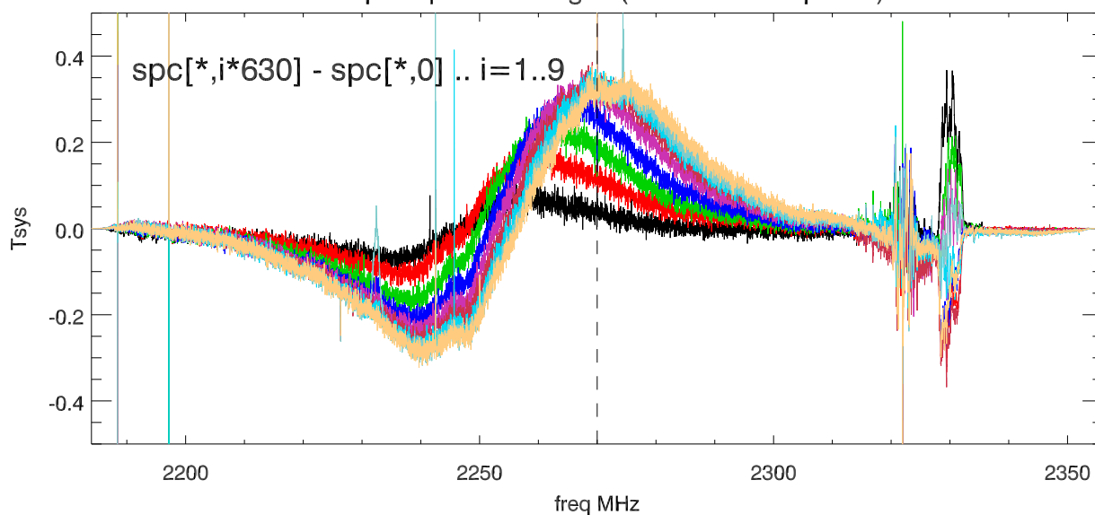
Overplot spectra changee (relative to 1st spectra)
