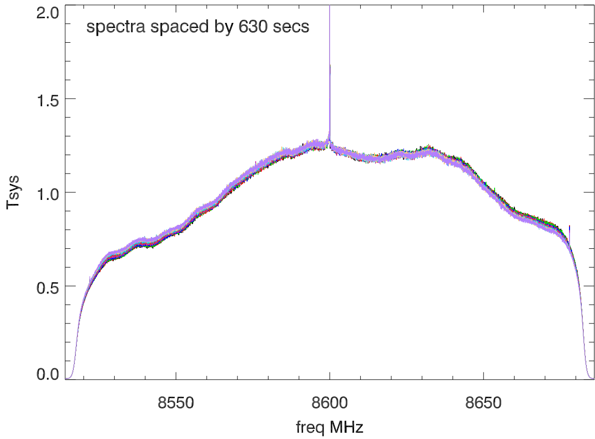
01mar16 p12m xband. Overplot 10 spectra (no offsets)
