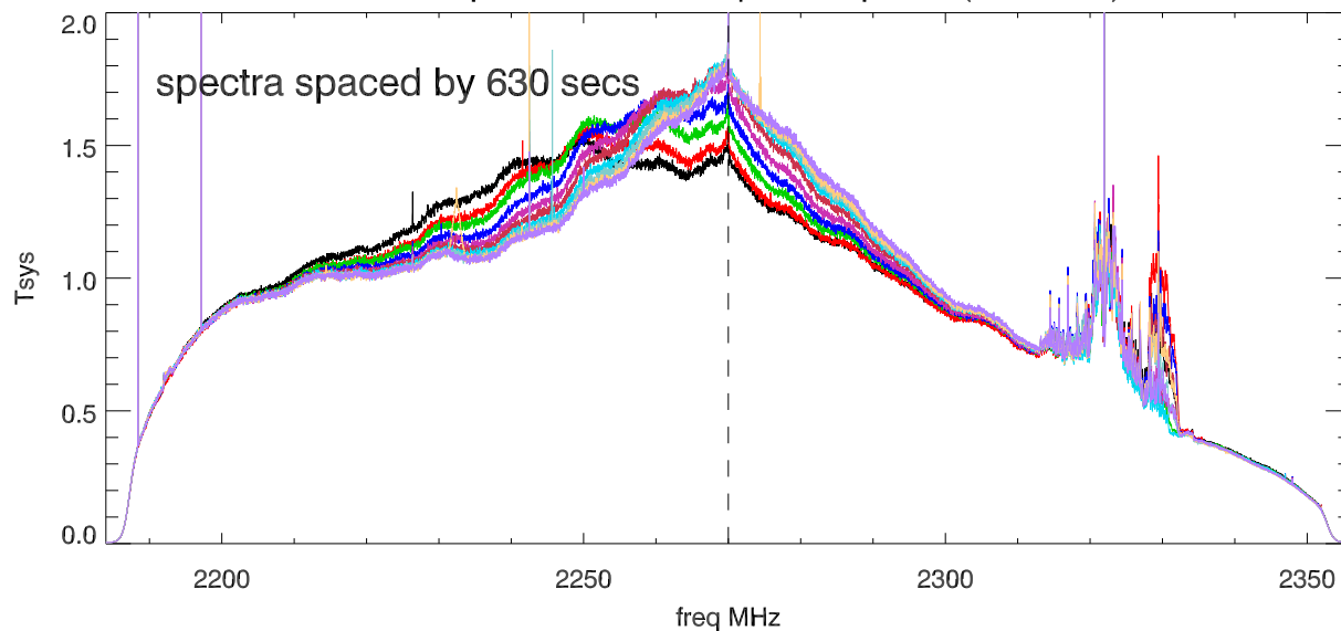
01mar16 p12m sband. Overplot 10 spectra (no offsets)
