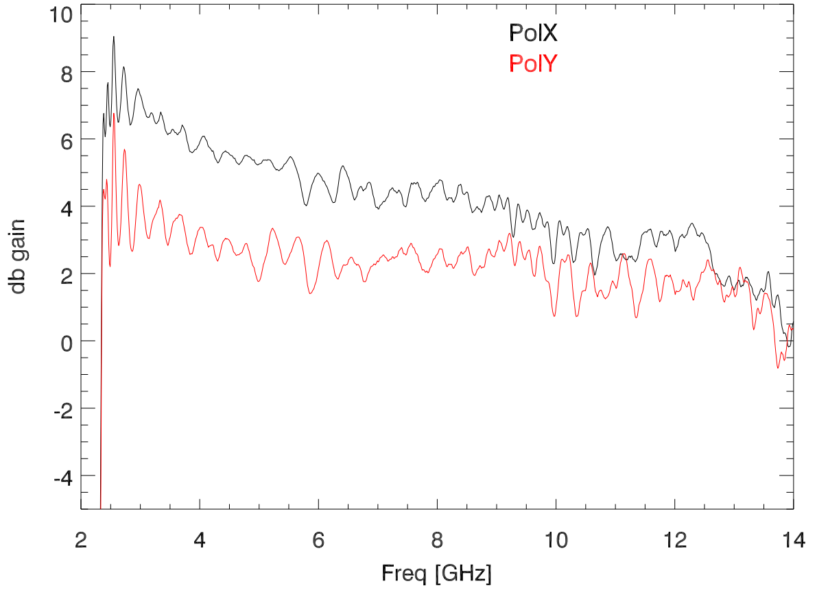
10feb23 S21 vs freq (input cal connetor,output lna)
