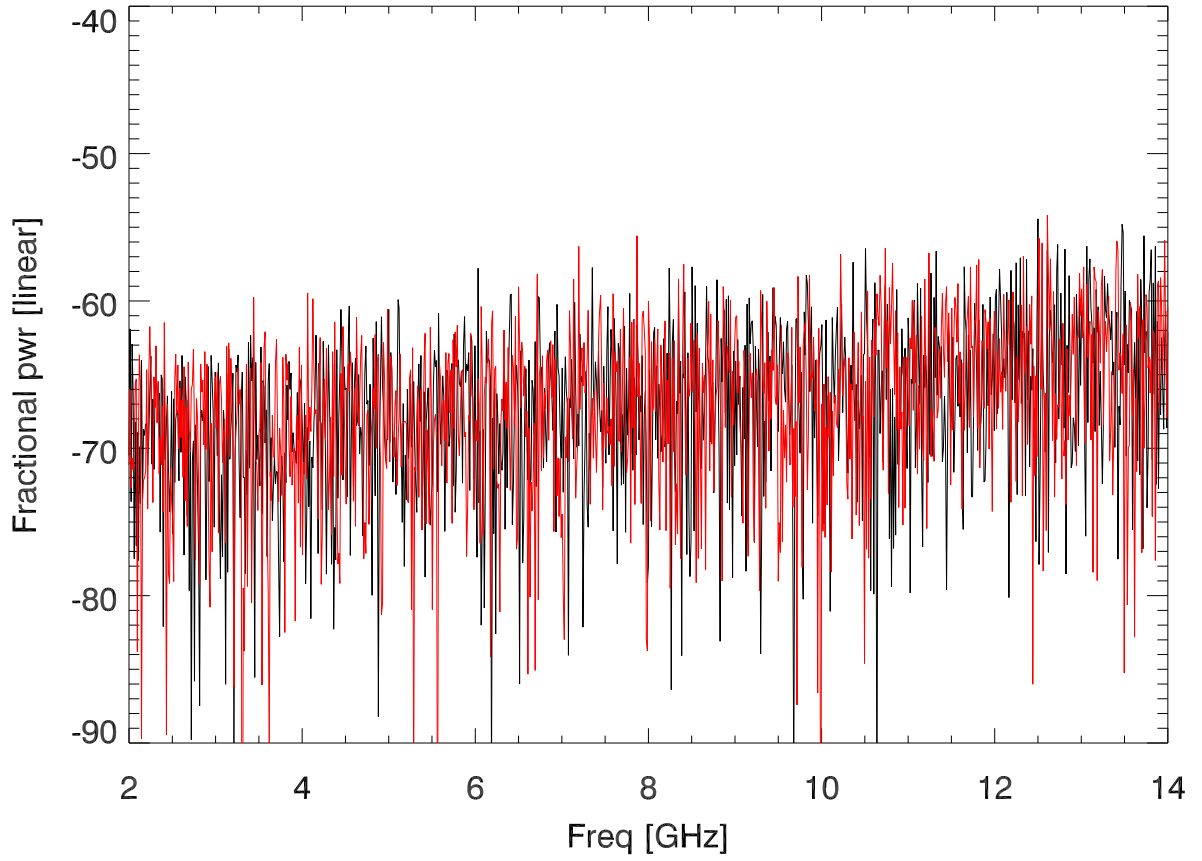
S12 vs freq. (Ina output to cal input)
