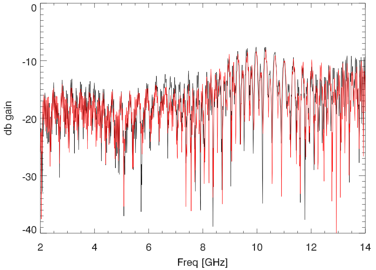
S11 vs freq. (reflected from cal input)
