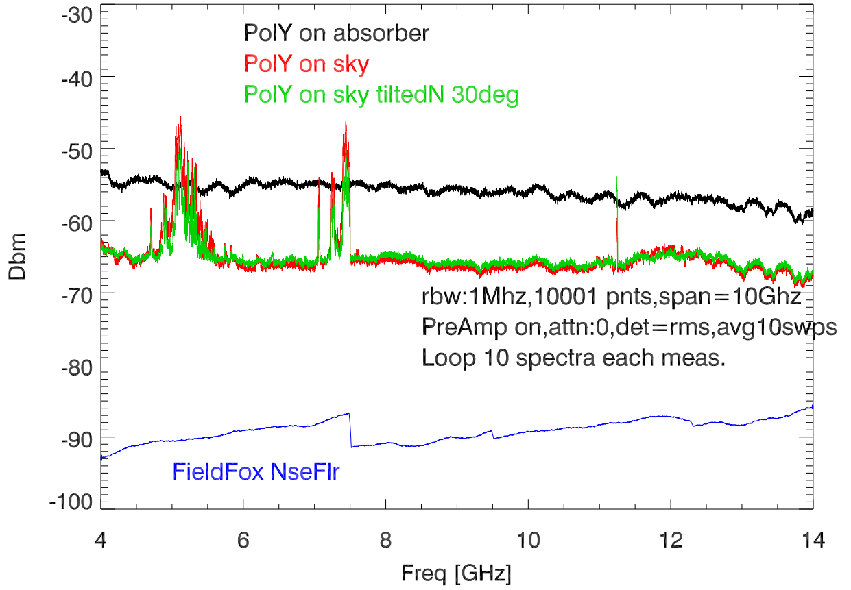
31jan23 wbRcv spectra at test range.
