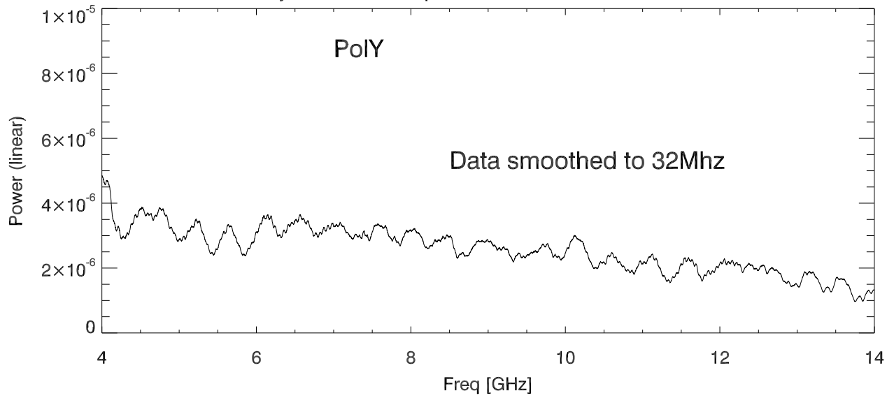
31jan23 cooled qrfh antTestBld. Power on Abs
