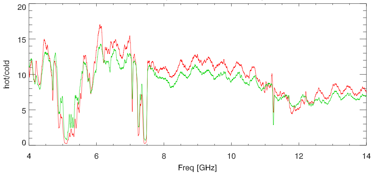
Yfactor (PowerHot/PowerCold)
