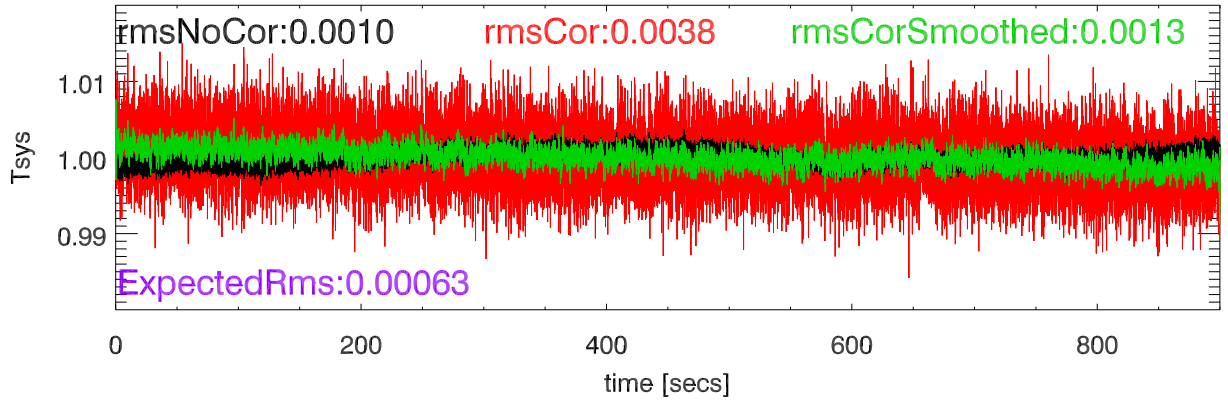
16jmar2 rms 16millisec totPwr (155Mhz bw). 8789PoIA
