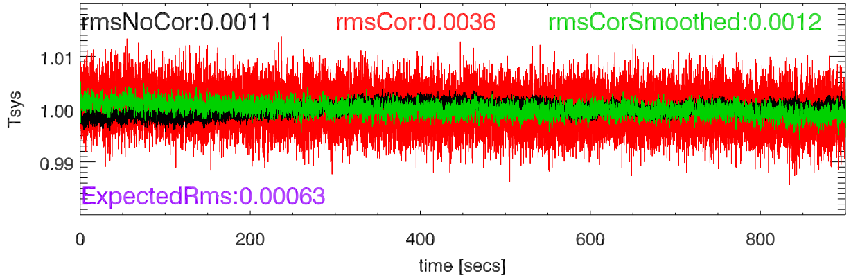
16jmar2 rms 16millisec totPwr (155Mhz bw). 8505PoIA
