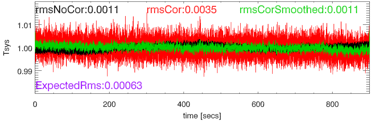
16jmar2 rms 16millisec totPwr (155Mhz bw). 8219PoIA
