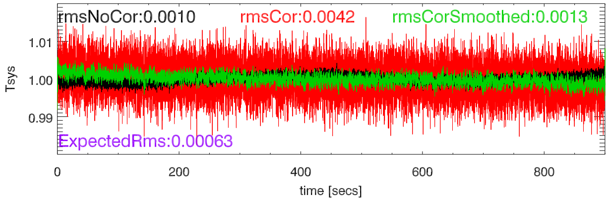
16jmar2 rms 16millisec totPwr (155Mhz bw). 9073PoIA
