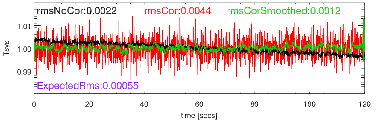
17jan22 rms 16millisec totPwr (165Mhz bw). 9072PoIA
