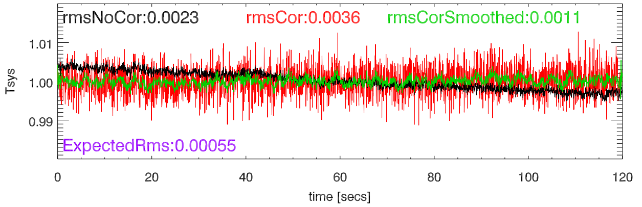
17jan22 rms 16millisec totPwr (165Mhz bw). 8504PoIA
