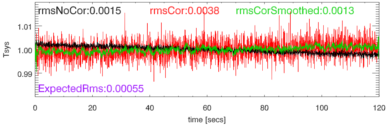
17jan22 rms 16millisec totPwr (165Mhz bw). 8788PoIA
