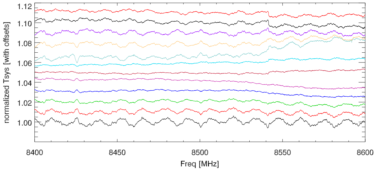
Blowup spectra 8400 to 8600 Mhz. Normalize to each hour
