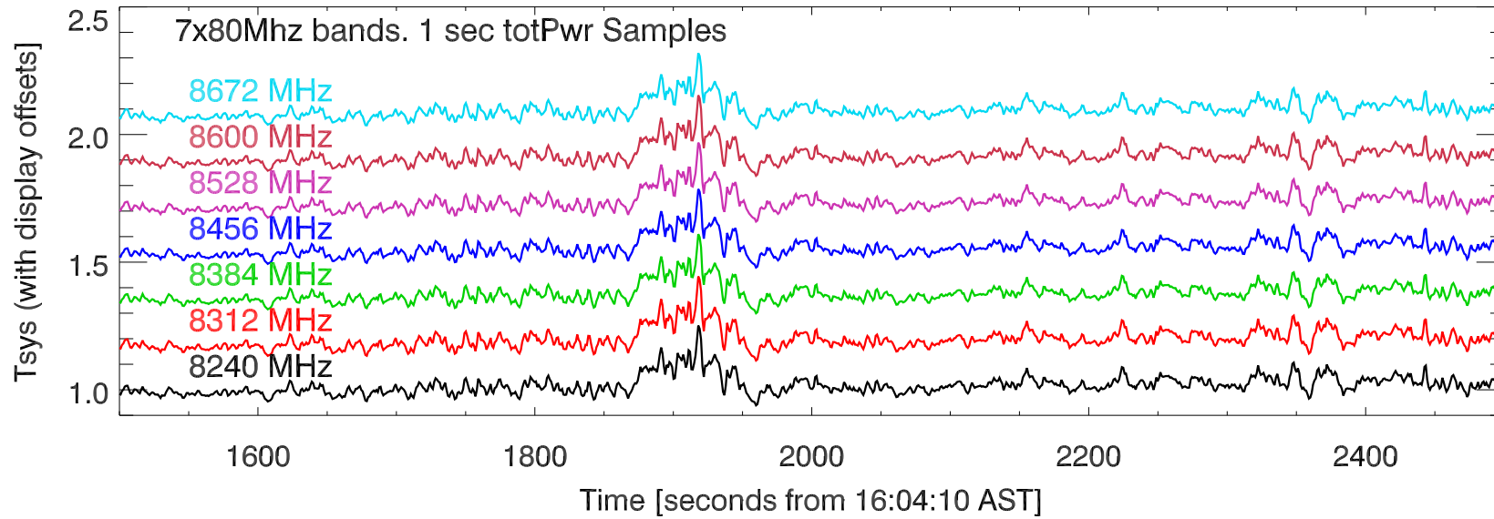
07jul21 12meter xb. totPwr vs time tracking sun for 1 hour PoIA (Blowup)
