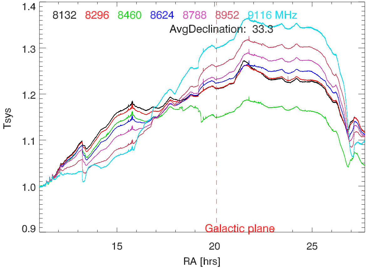
210701 12m totalPwr(172MHz) vs RA. OverplotBands. PolA
