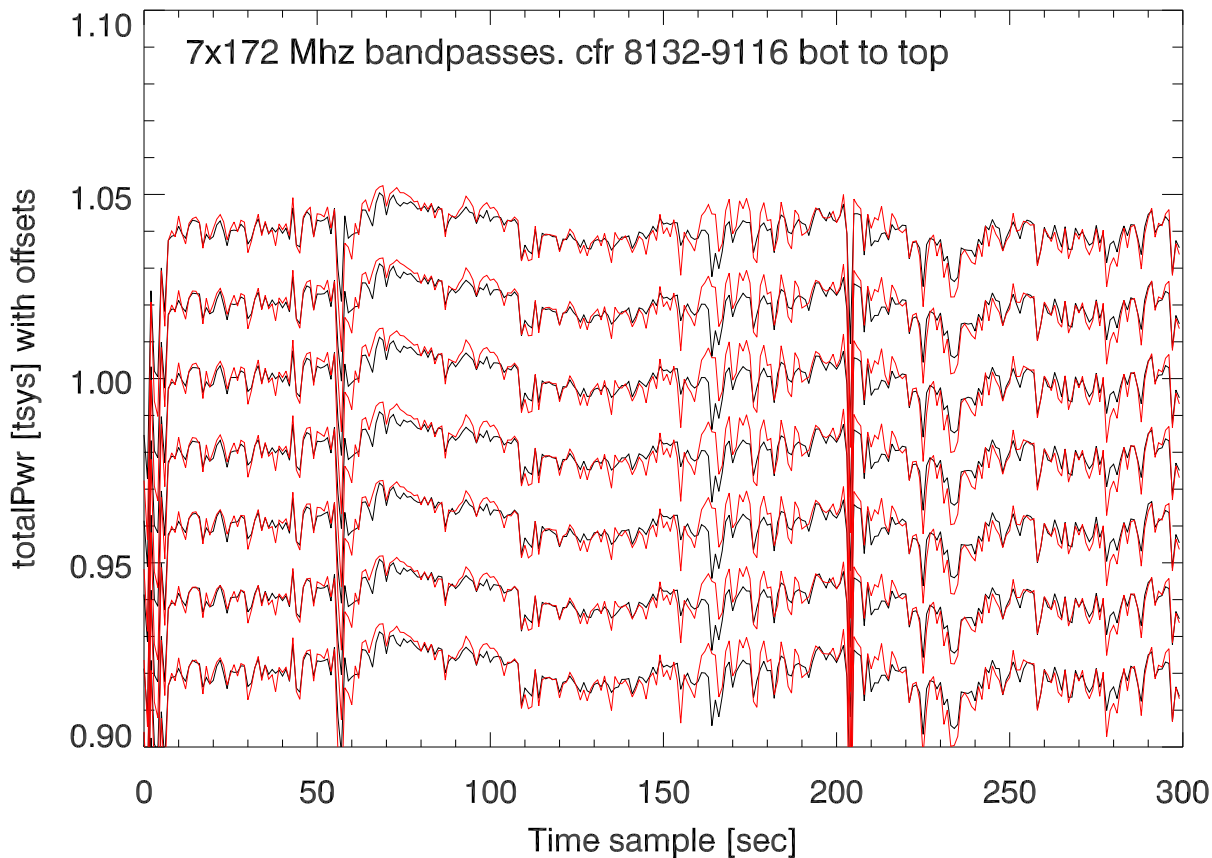
210324 p12m xb. TotPwr vs time for scan starting at:19:29:03
