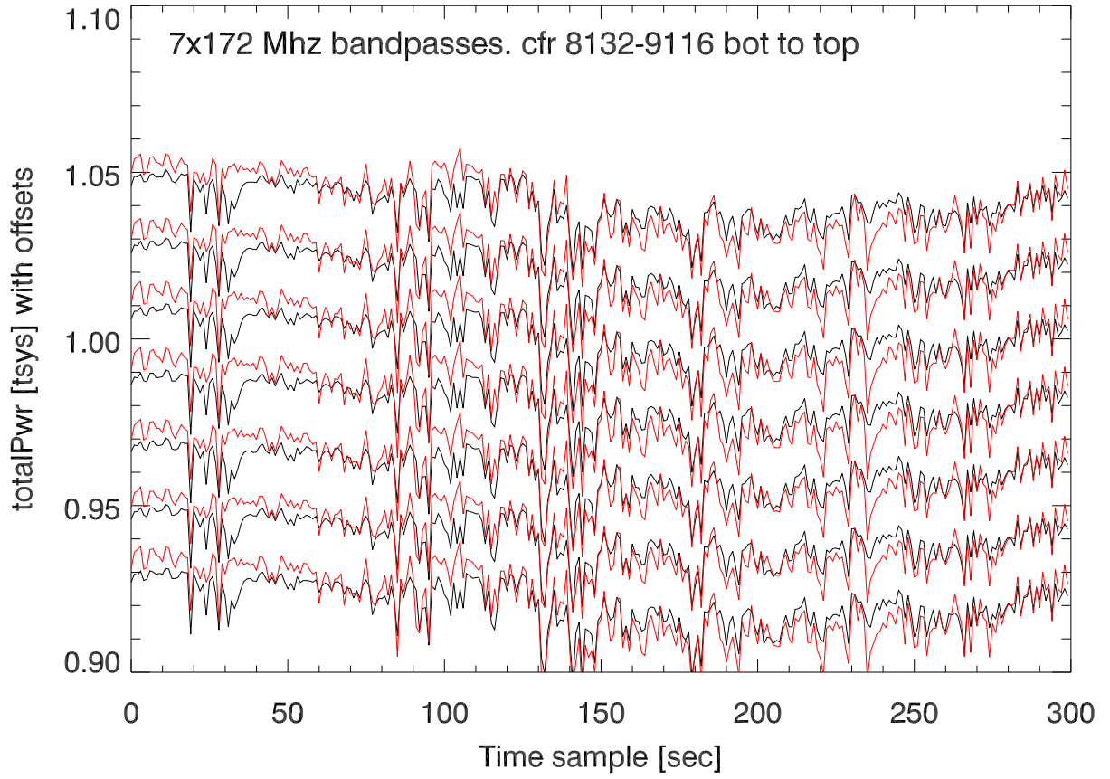
210324 p12m xb. TotPwr vs time for scan starting at:19:54:33
