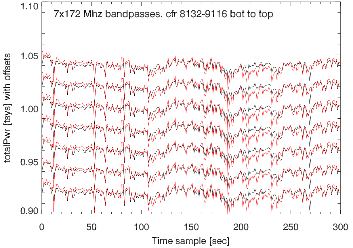
210324 p12m xb. TotPwr vs time for scan starting at:19:39:15
