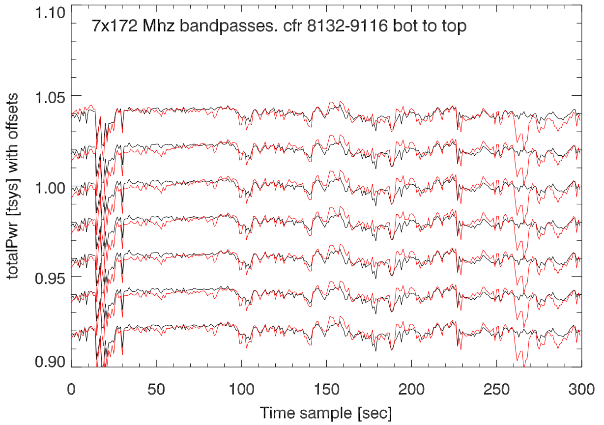
210324 p12m xb. TotPwr vs time for scan starting at:19:02:21
