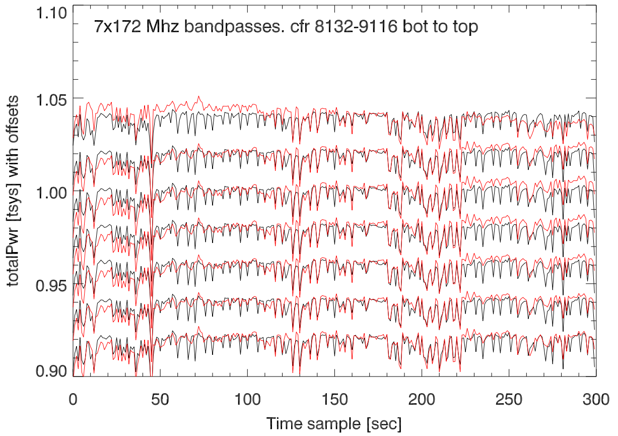
210324 p12m xb. TotPwr vs time for scan starting at:18:57:15
