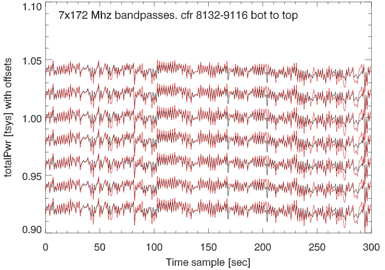
210324 p12m xb. TotPwr vs time for scan starting at:19:59:39
