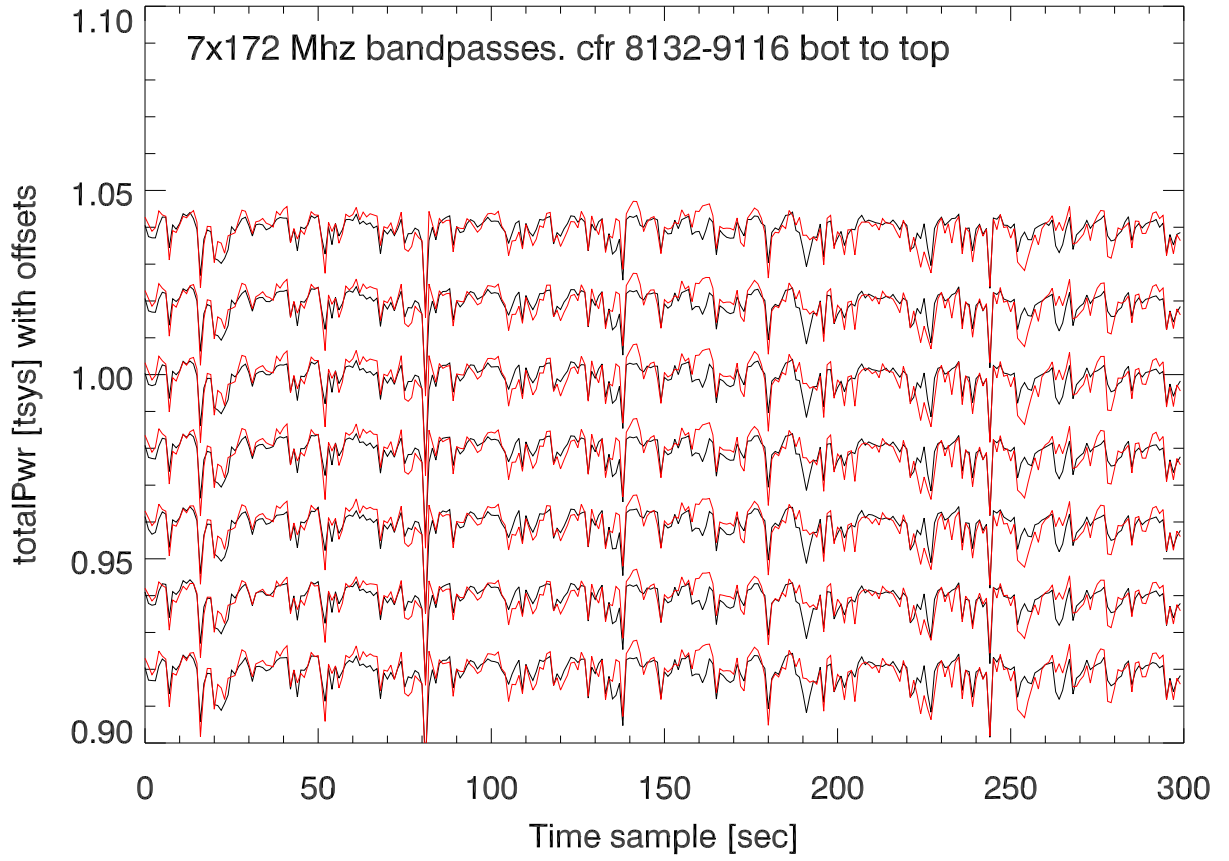
210324 p12m xb. TotPwr vs time for scan starting at:19:44:21
