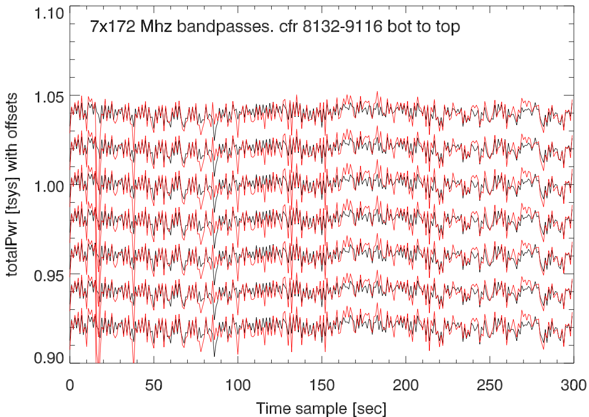
210324 p12m xb. TotPwr vs time for scan starting at:20:04:45
