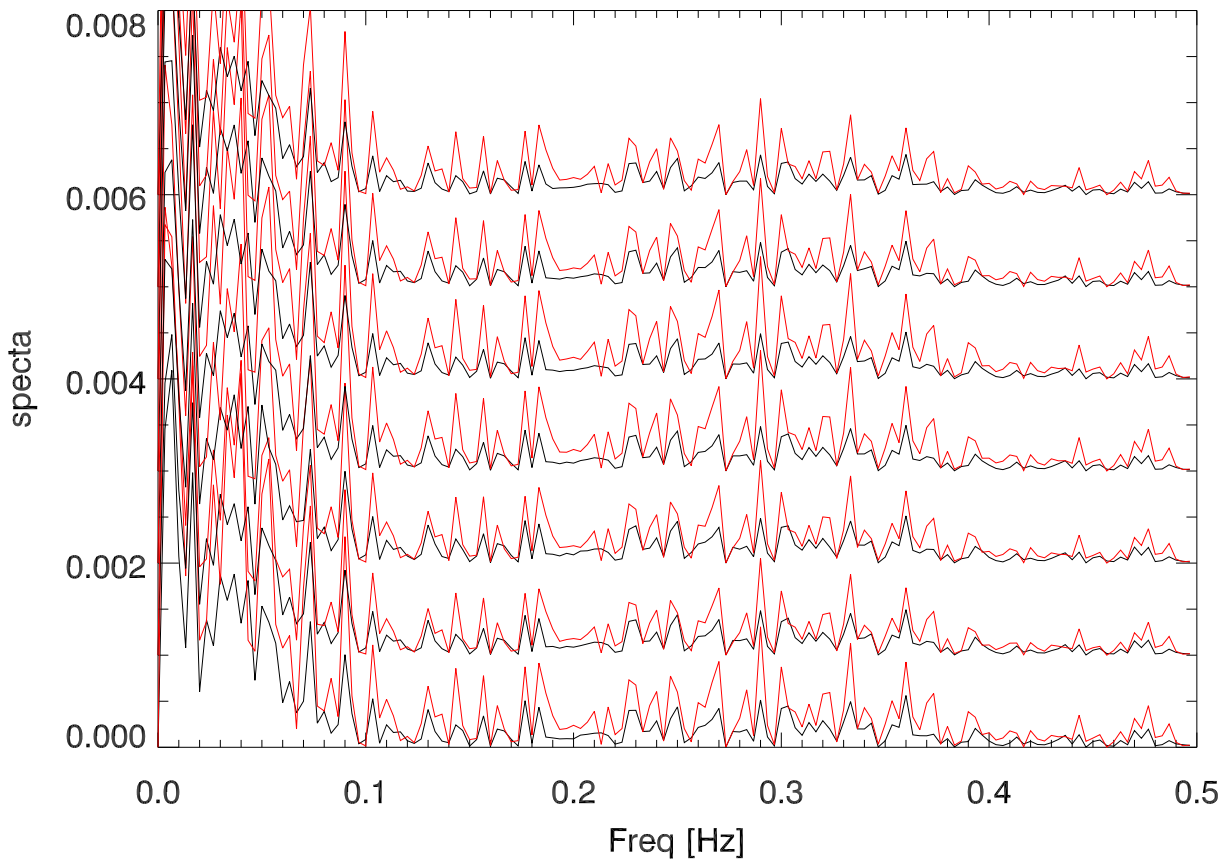
Spectra of total power (1 sec samples)
