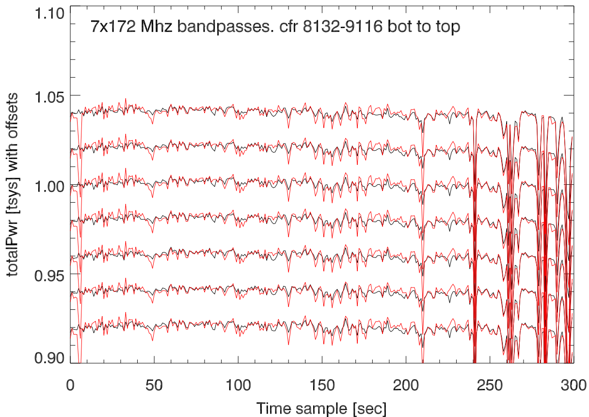
210324 p12m xb. TotPwr vs time for scan starting at:19:23:57
