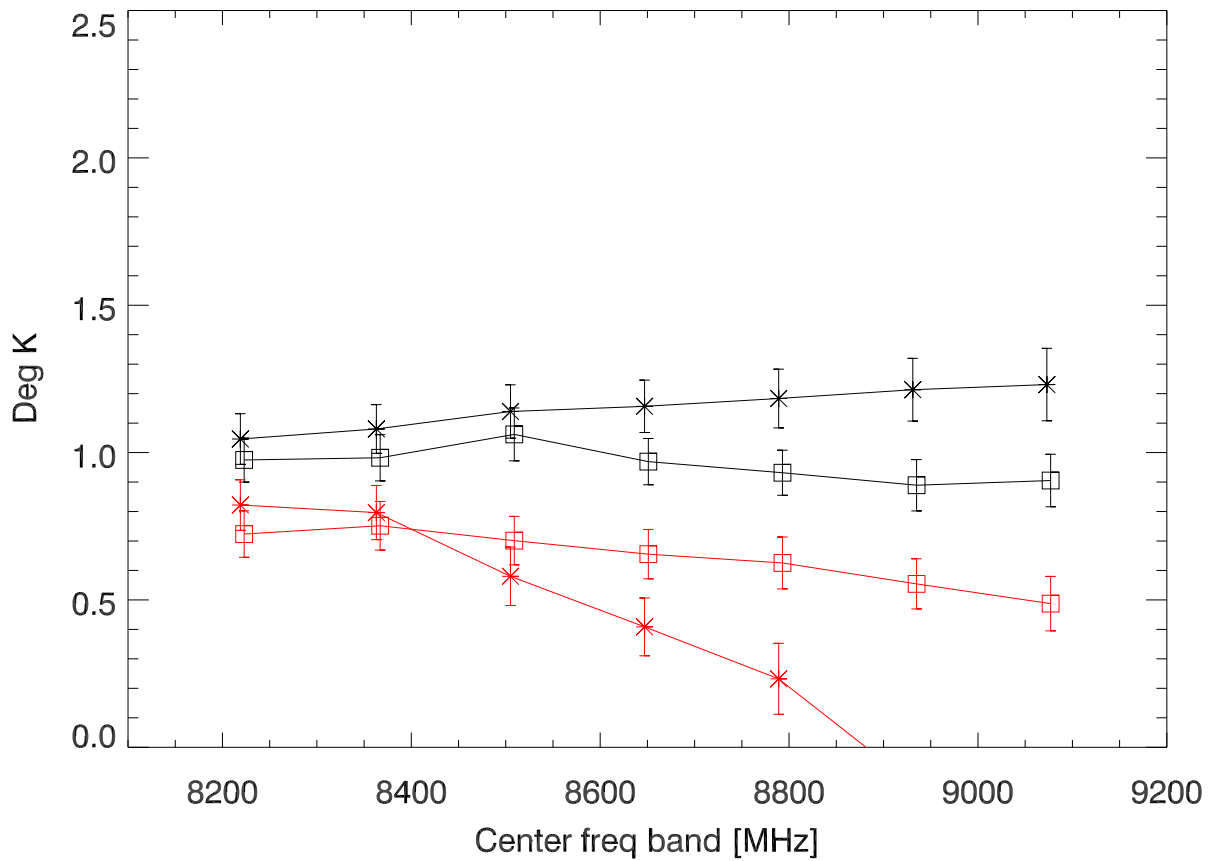
220819 SrcDeflection by freq Band. source:3C274 noCor
