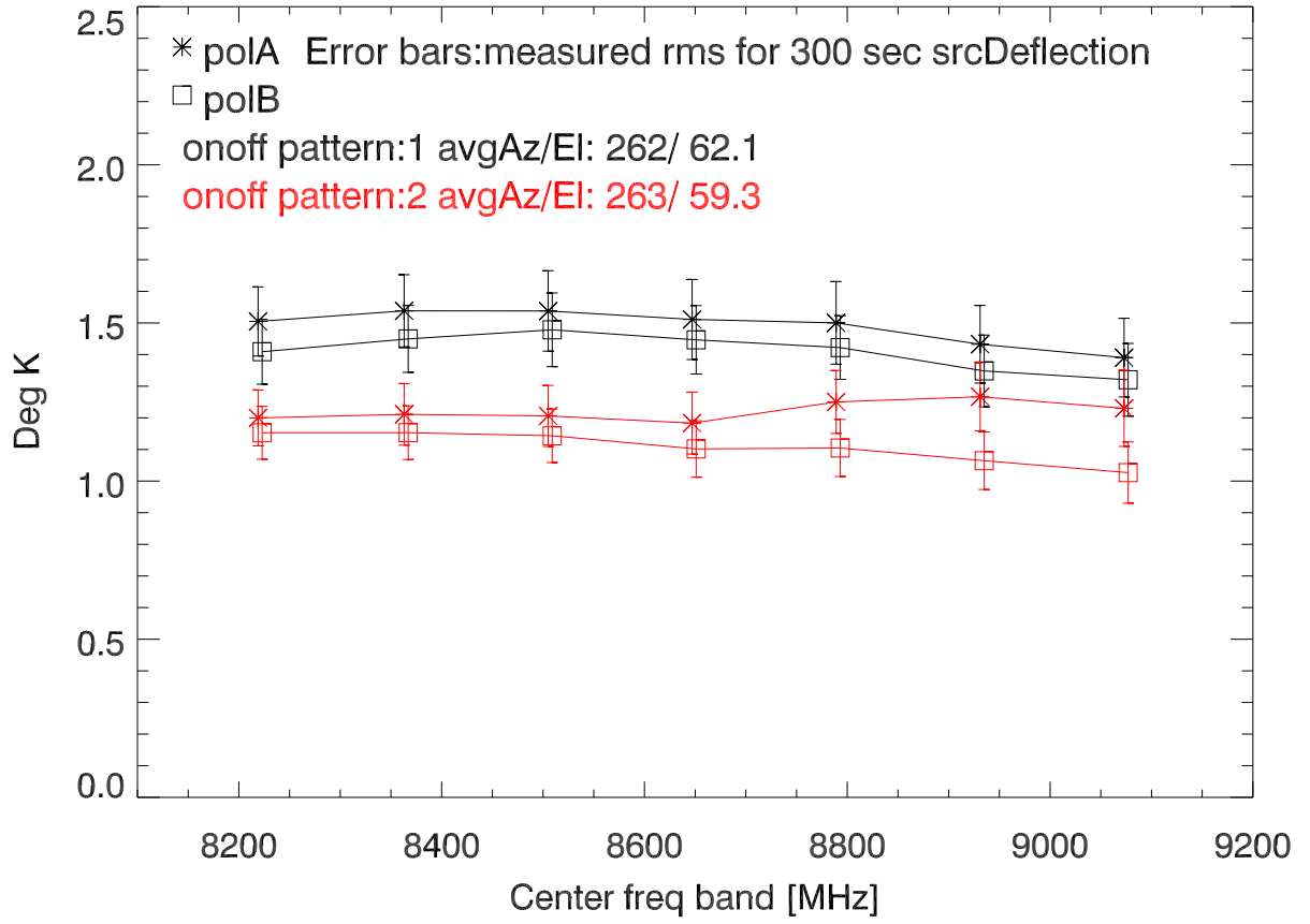
220819 SrcDeflection by freq Band. source:3C274 Cor
