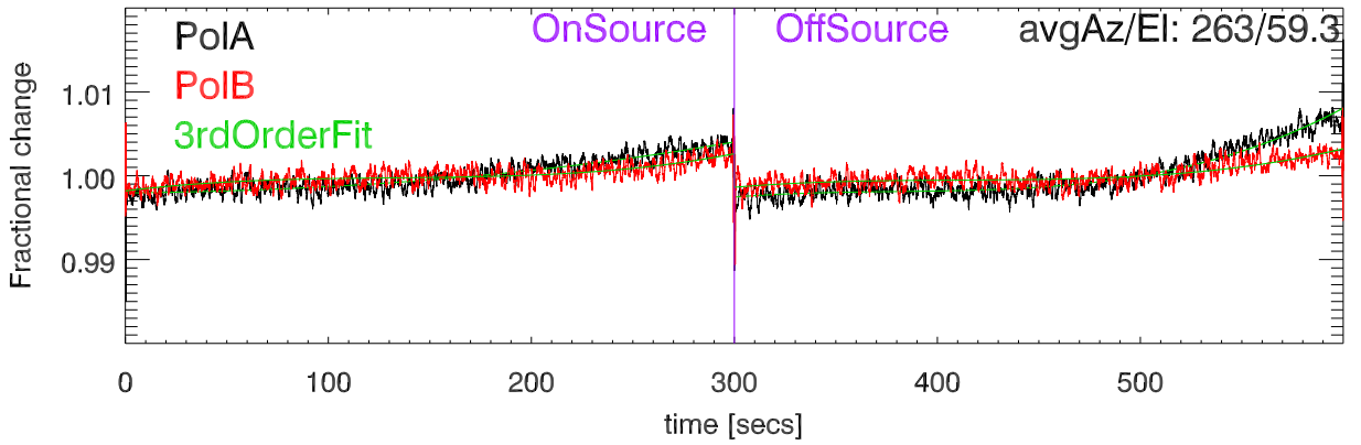
220819 3C274 Fractional change cal Deflection vs time. BandCfr:8647.0 Pat:2
