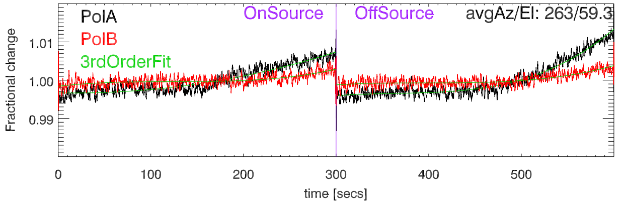
220819 3C274 Fractional change cal Deflection vs time. BandCfr:8931.0 Pat:2
