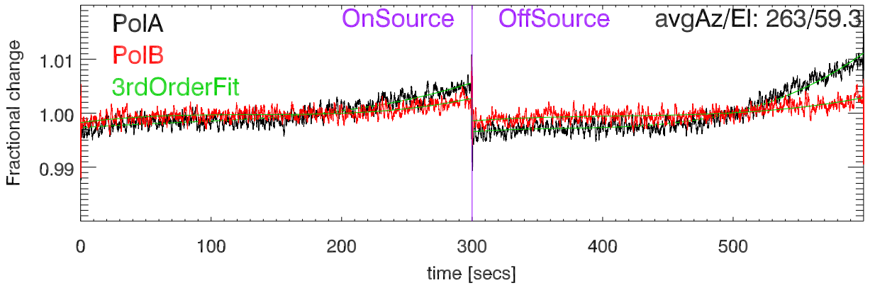
220819 3C274 Fractional change cal Deflection vs time. BandCfr:8789.0 Pat:2
