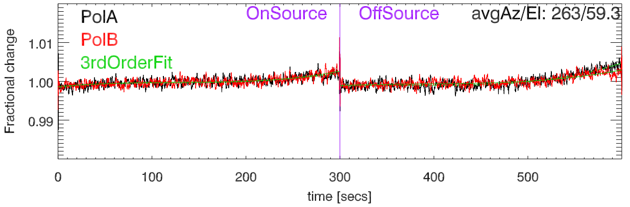
220819 3C274 Fractional change cal Deflection vs time. BandCfr:8363.0 Pat:2
