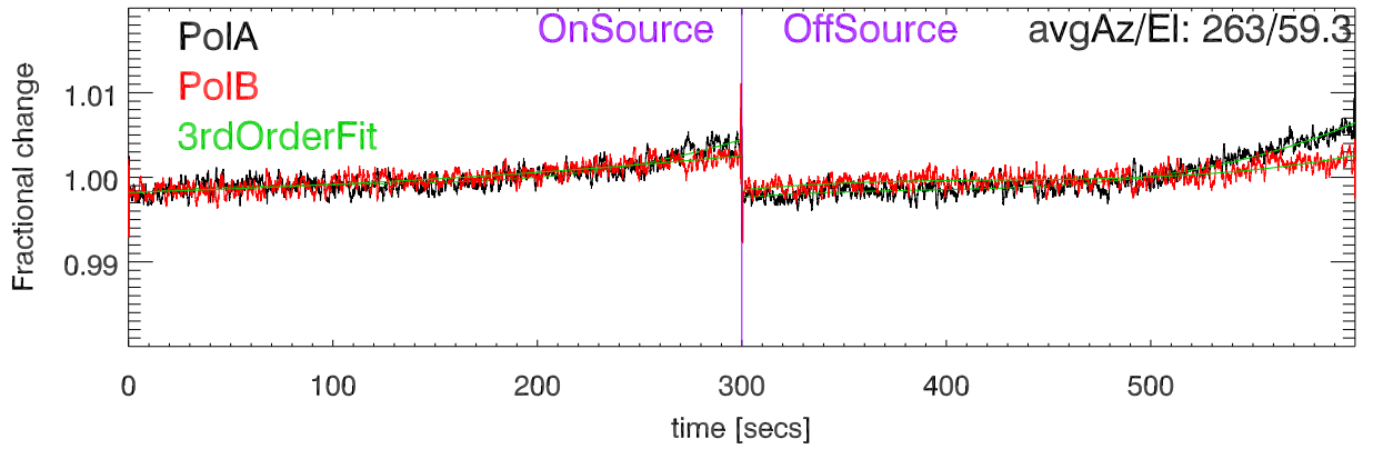
220819 3C274 Fractional change cal Deflection vs time. BandCfr:8505.0 Pat:2
