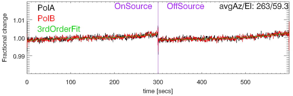
220819 3C274 Fractional change cal Deflection vs time. BandCfr:8219.0 Pat:2
