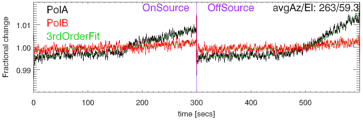
220819 3C274 Fractional change cal Deflection vs time. BandCfr:9073.0 Pat:2
