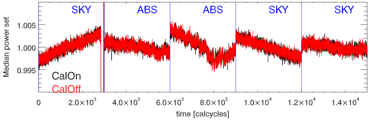
220117 measureCal totPwrVsTm. 8789 Mhz PoIA
