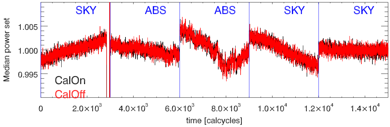
220117 measureCal totPwrVsTm. 8219 Mhz PoIA
