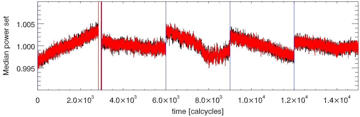
8931 Mhz PoIA
