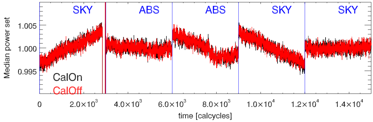
220117 measureCal totPwrVsTm. 9073 Mhz PoIA
