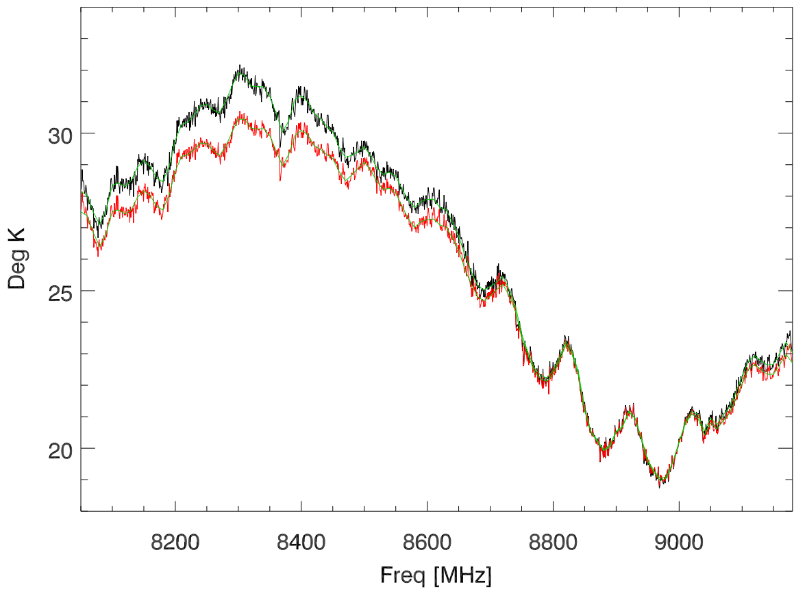
230620 Tcal vs freq for filt 6: 8050-9180Mhz PoIB
