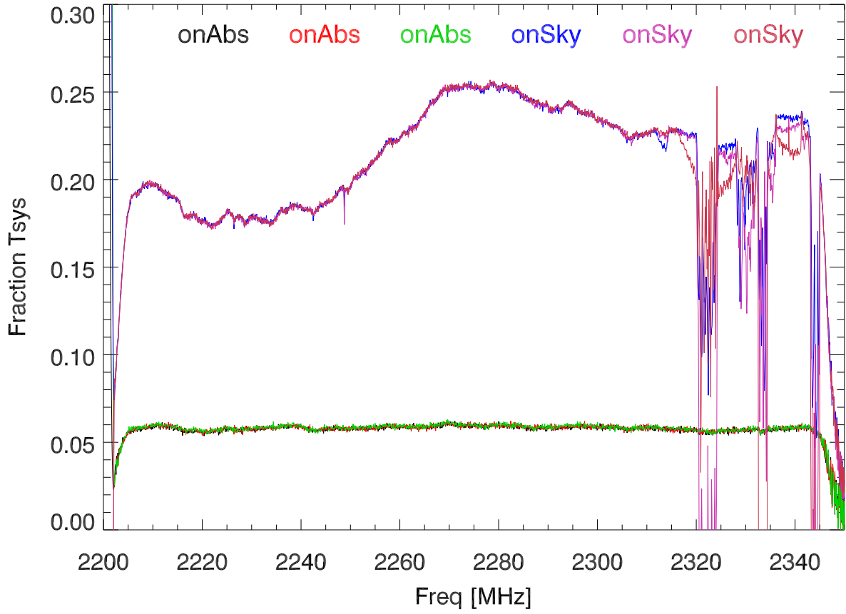
220624 CalDeflection/CalOff vs freq. PoIA
