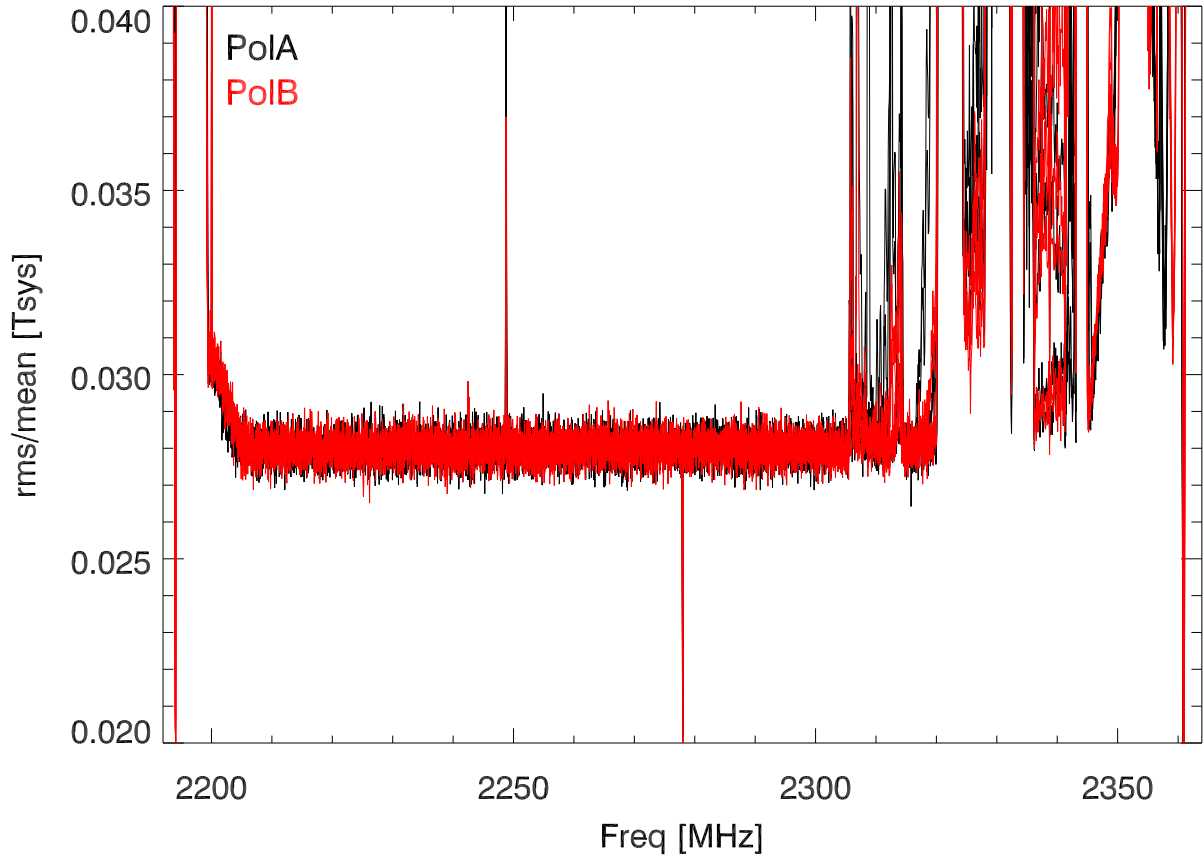
220624 Rms/mean by freqChan for calon,caloff spectra. OnSky
