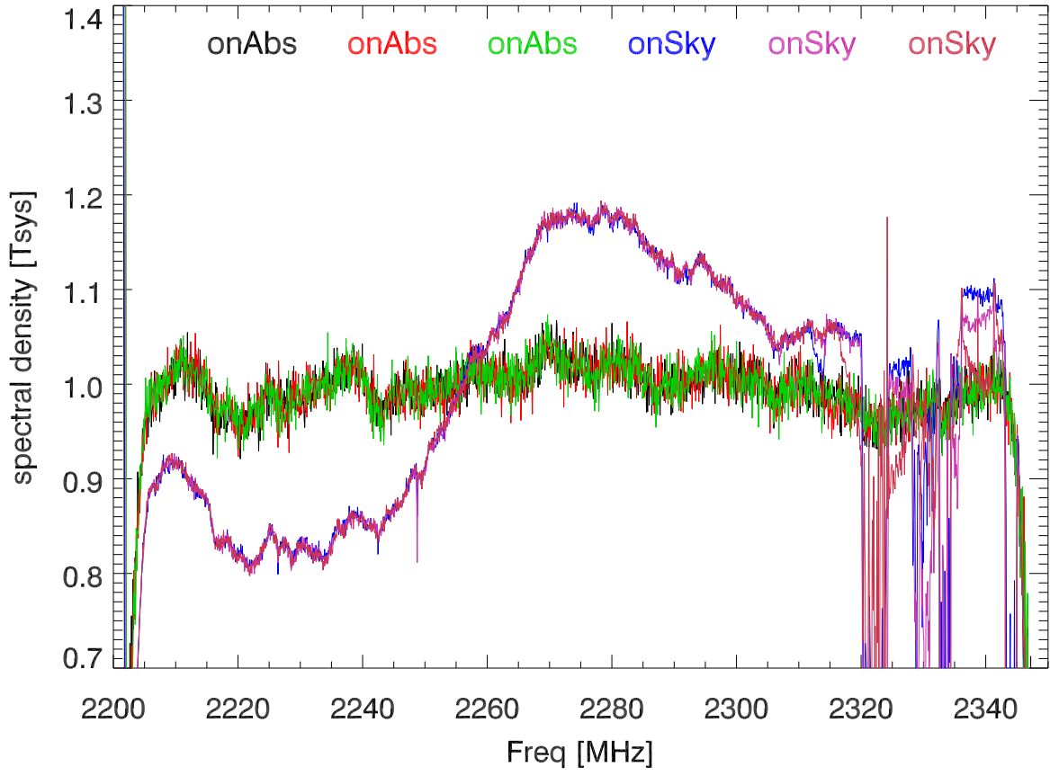
220624 Normalized CalDeflect/CalOff vs freq. PoIA
