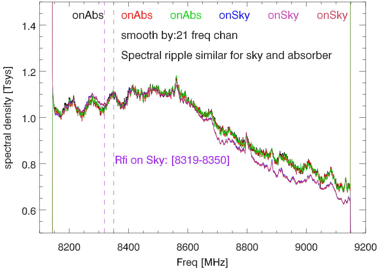
220607 Normalized CalDeflect/CalOff vs freq. PoIA
