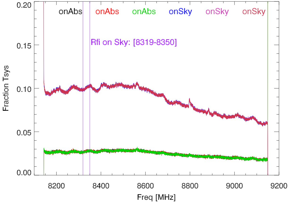
220607 CalDeflect/CalOff vs freq. PoIA
