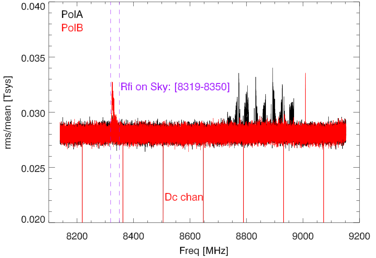
220607 Rms/mean by freqChan for calon,caloff spectra. OnSky
