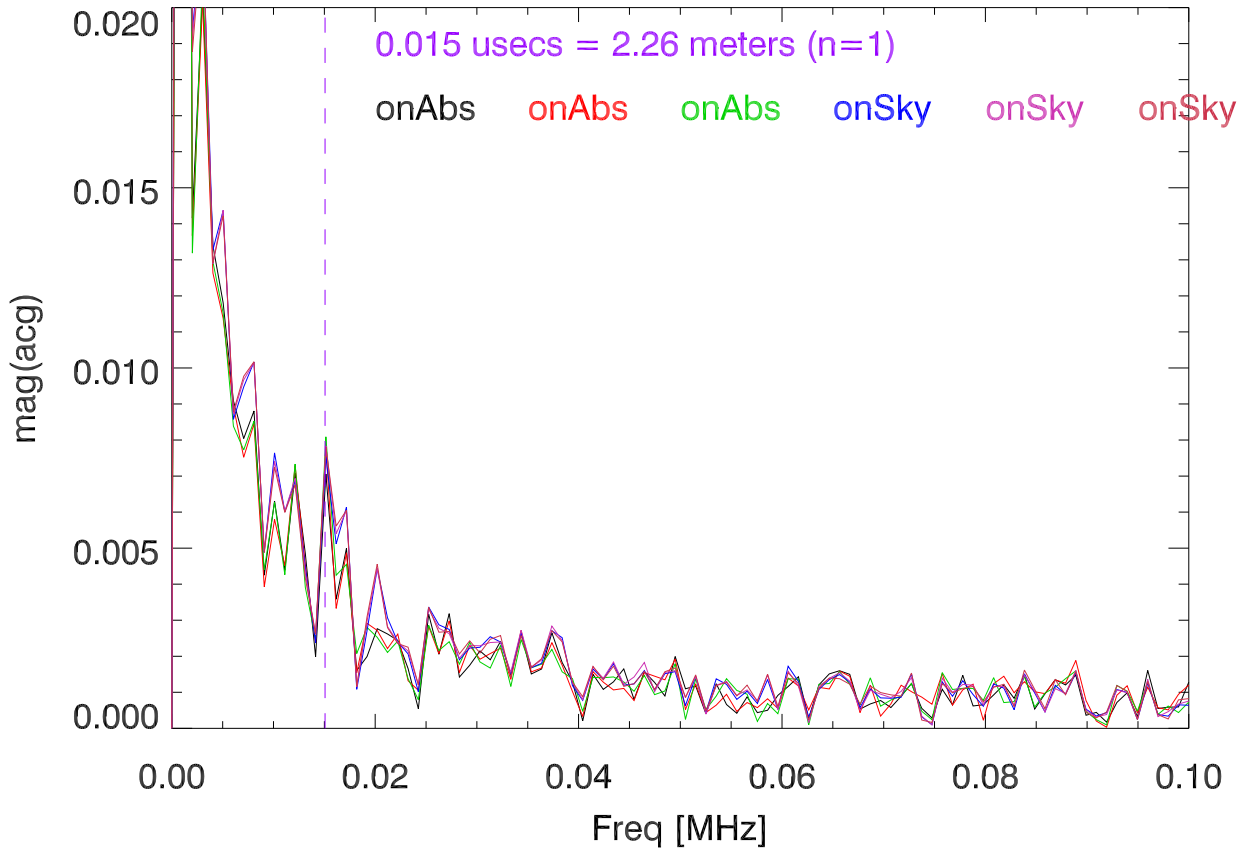
220607 acf of calRatio spectra showing ripple spacing. PoIA
