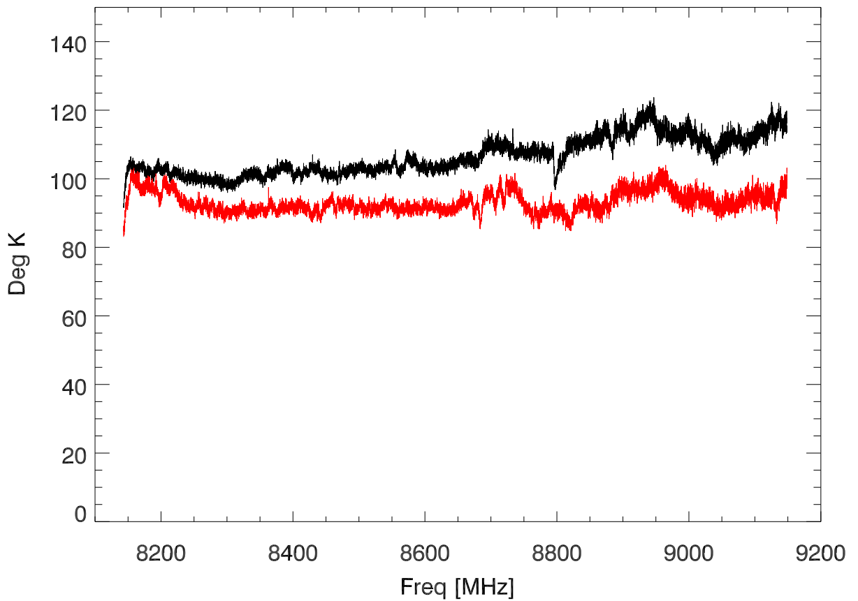
220607 Measured Tsys vs freq (using calOffs)
