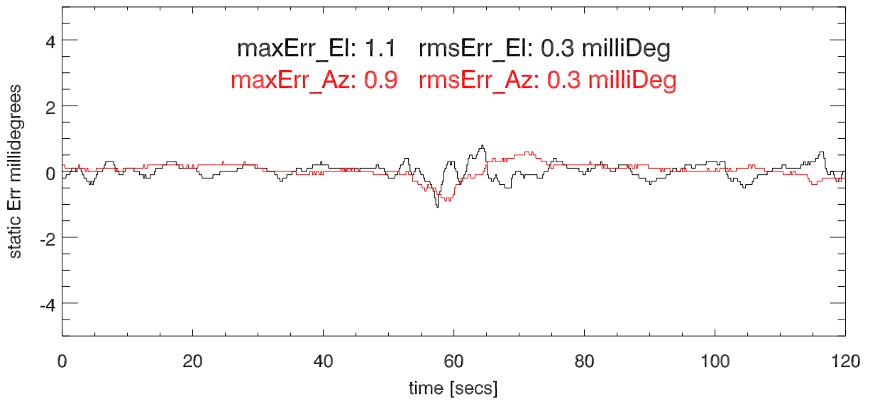
Static tracking error. el=45 deg
