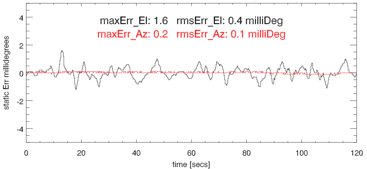
Static tracking error. el=80 deg
