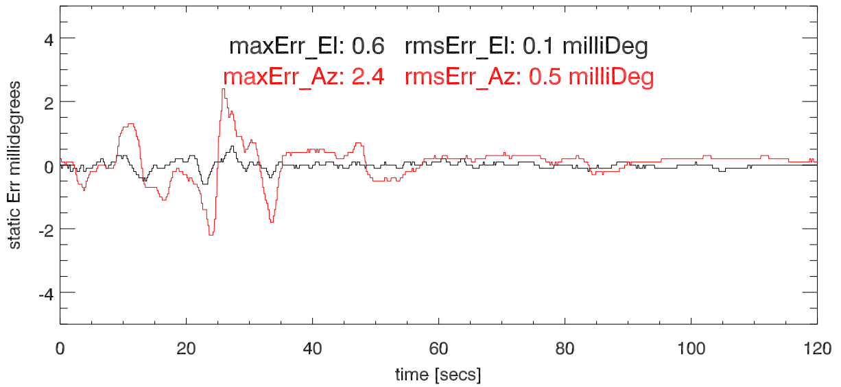
24jan11:Static tracking error. el=10 deg
