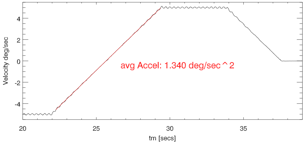
Az_vel vs Time: change vel -5 to +5 deg/sec at el=10deg
