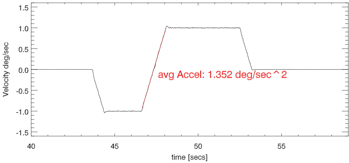
El_vel vs Time: change vel -1 to +1 deg/sec at el=10deg
