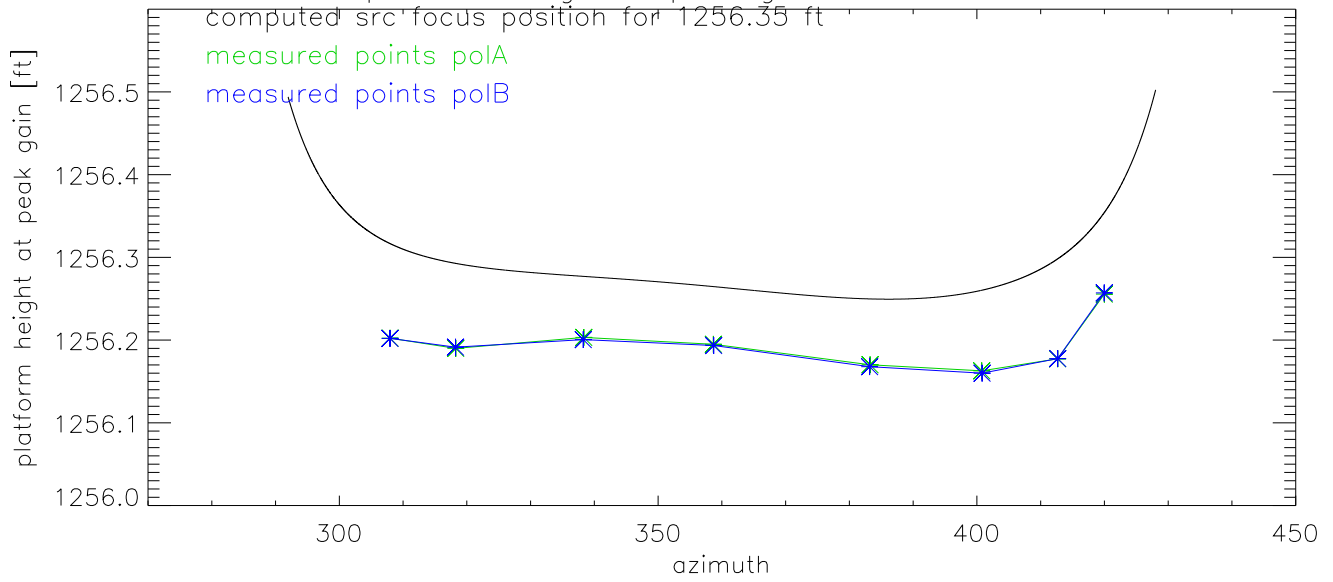
platform height at peak gain versus za
