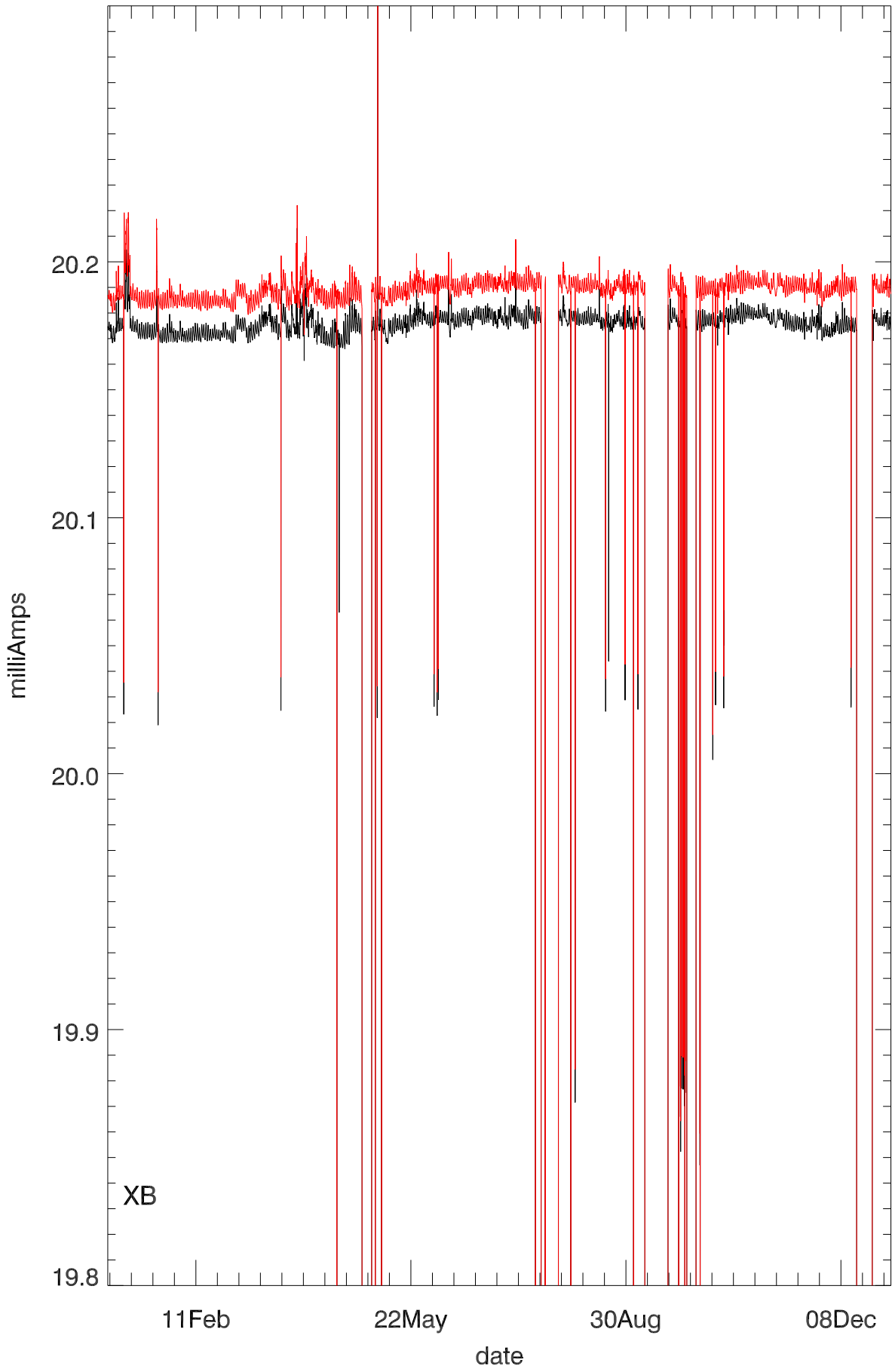
Dewar Current stage 1 (year 2014)
