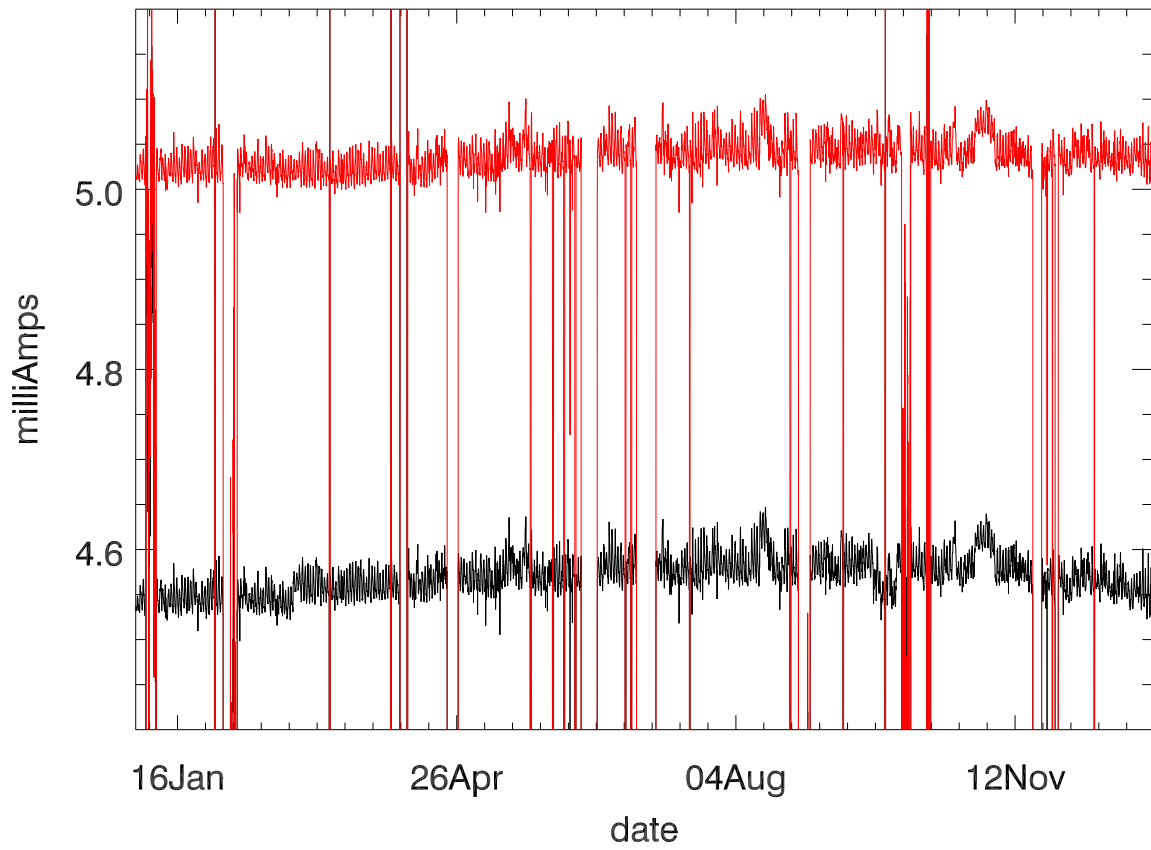
Dewar Current stage 1 (year 2019)
