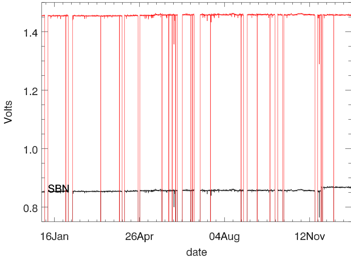
Dewar voltage stage 2 (year 2019)
