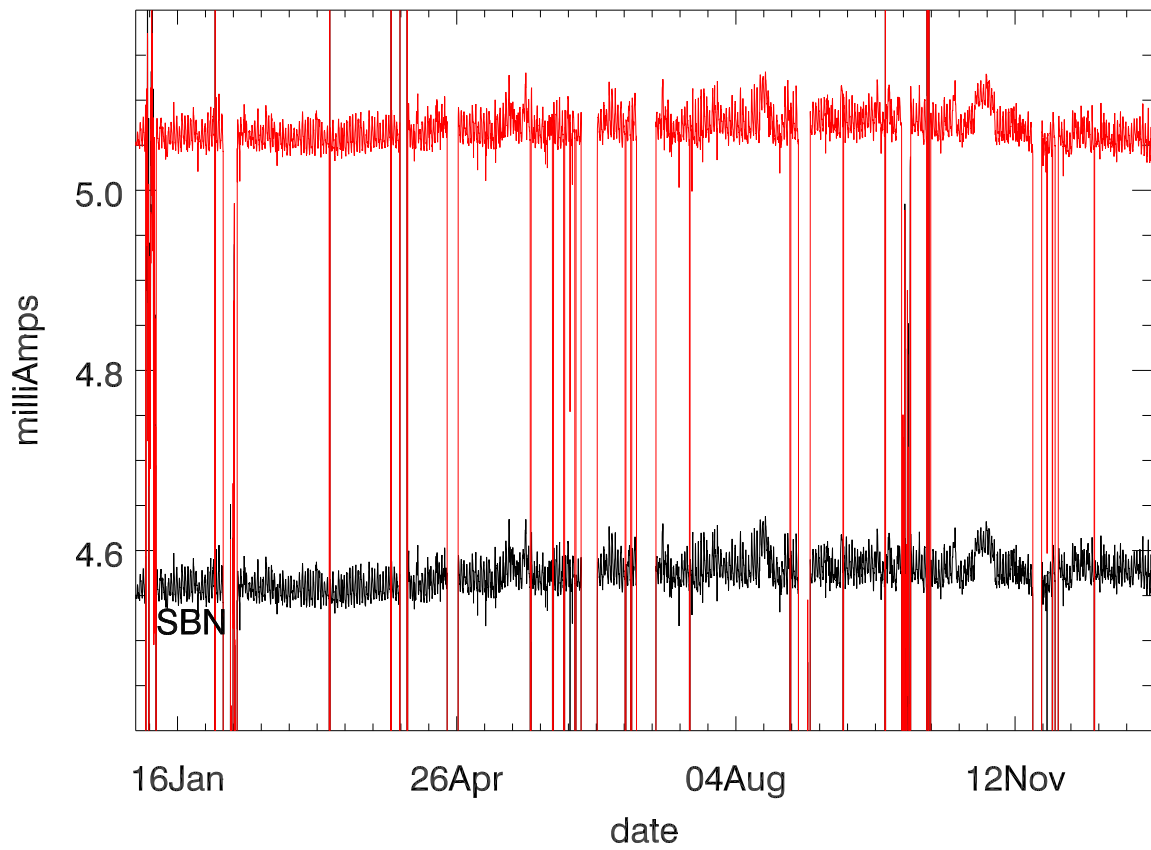
Dewar Current stage 2 (year 2019)
