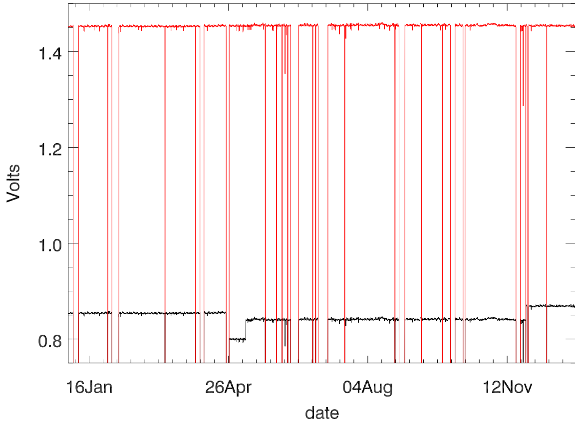
Dewar voltage stage 1 (year 2019)
