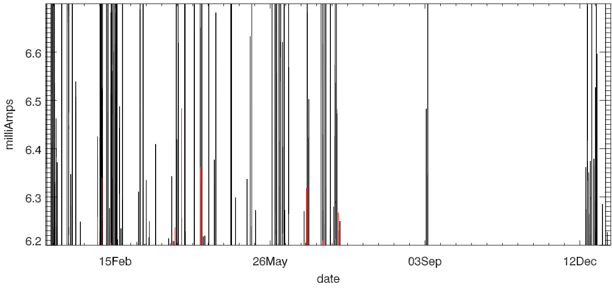
Dewar Current stage 1 (year 2017)
