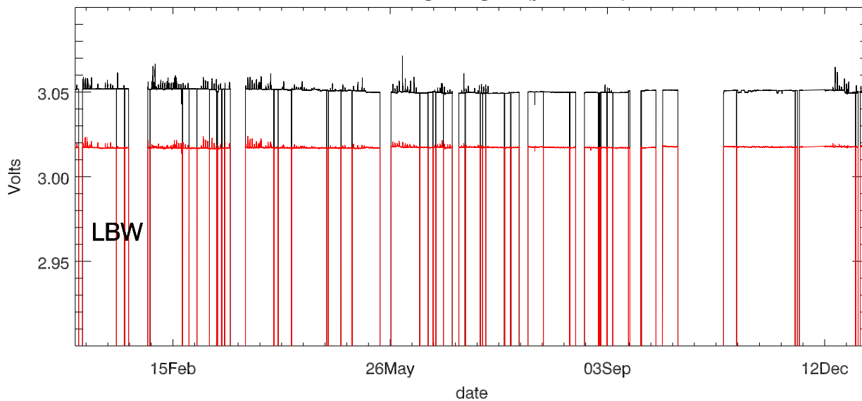
Dewar voltage stage 3 (year 2017)
