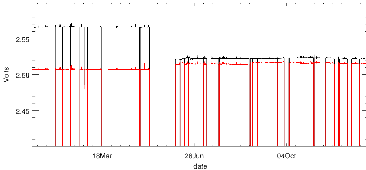
Dewar voltage stage 1 (year 2015)
