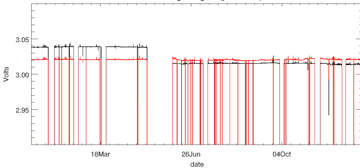
Dewar voltage stage 2 (year 2015)
