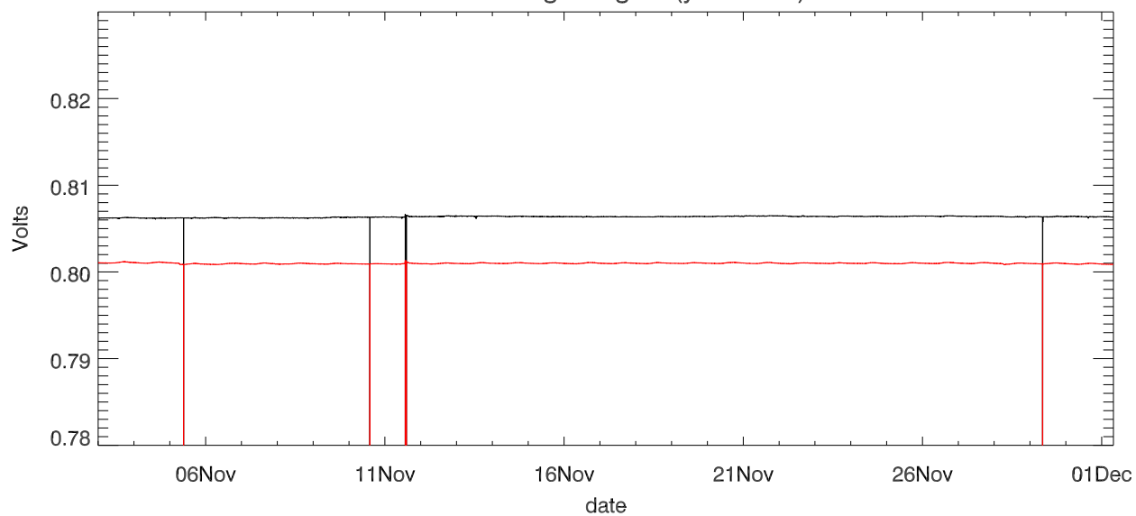
Dewar voltage stage 2 (year 2020)
