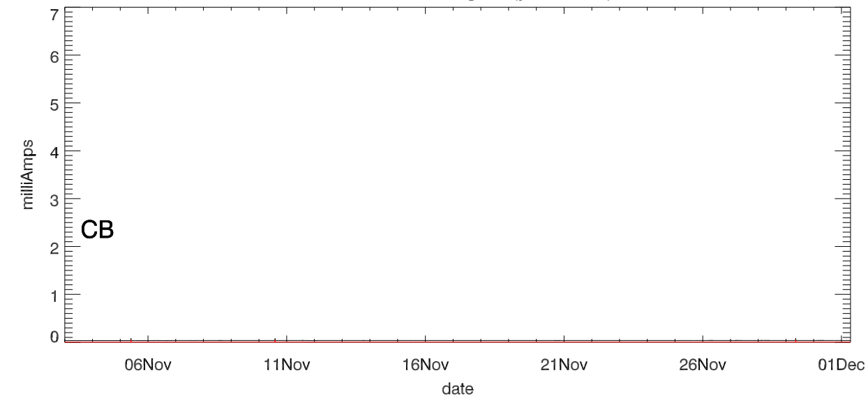
Dewar Current stage 3 (year 2020)
