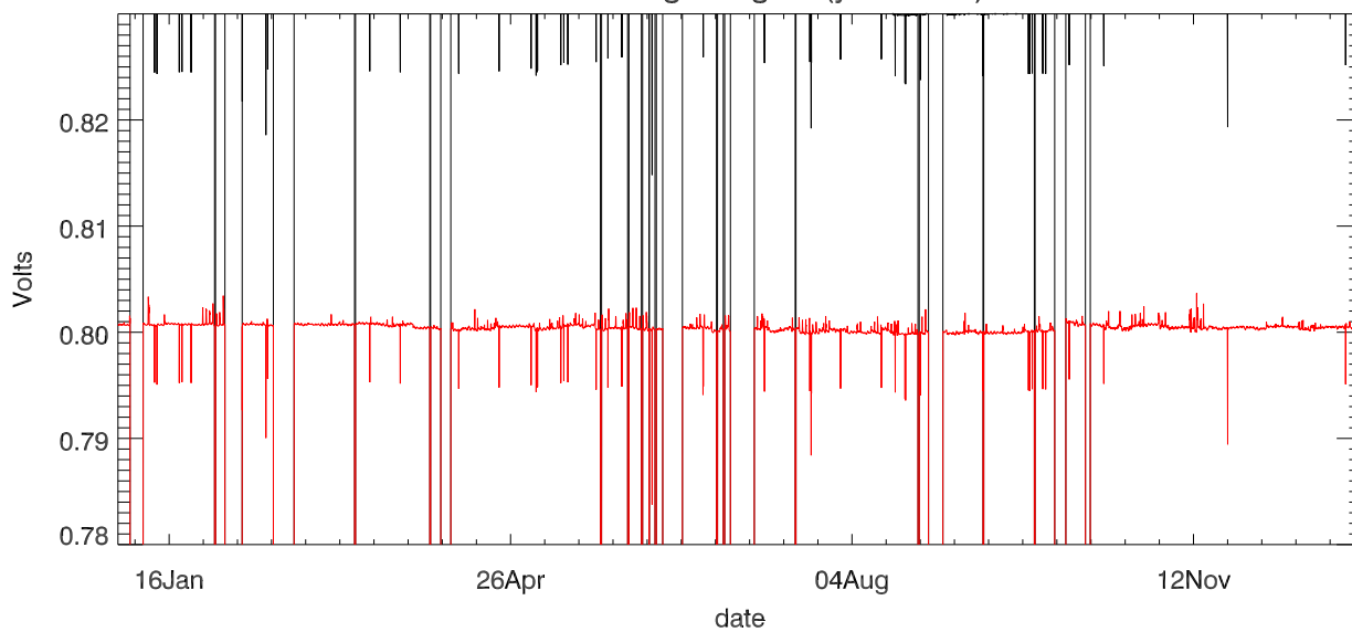
Dewar voltage stage 2 (year 2019)
