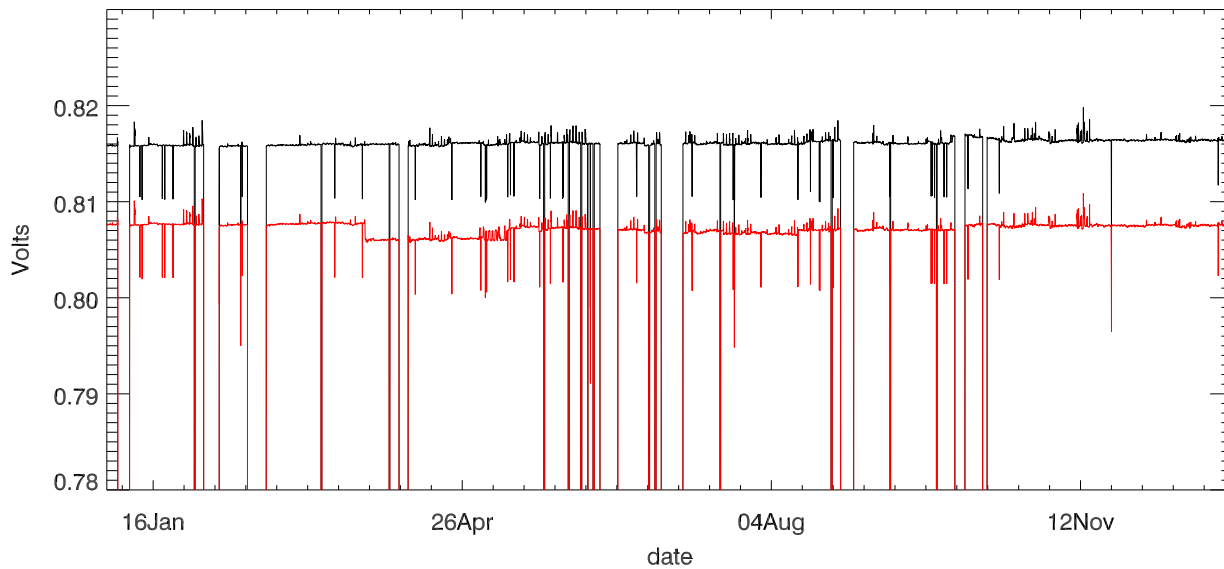
Dewar voltage stage 1 (year 2019)
