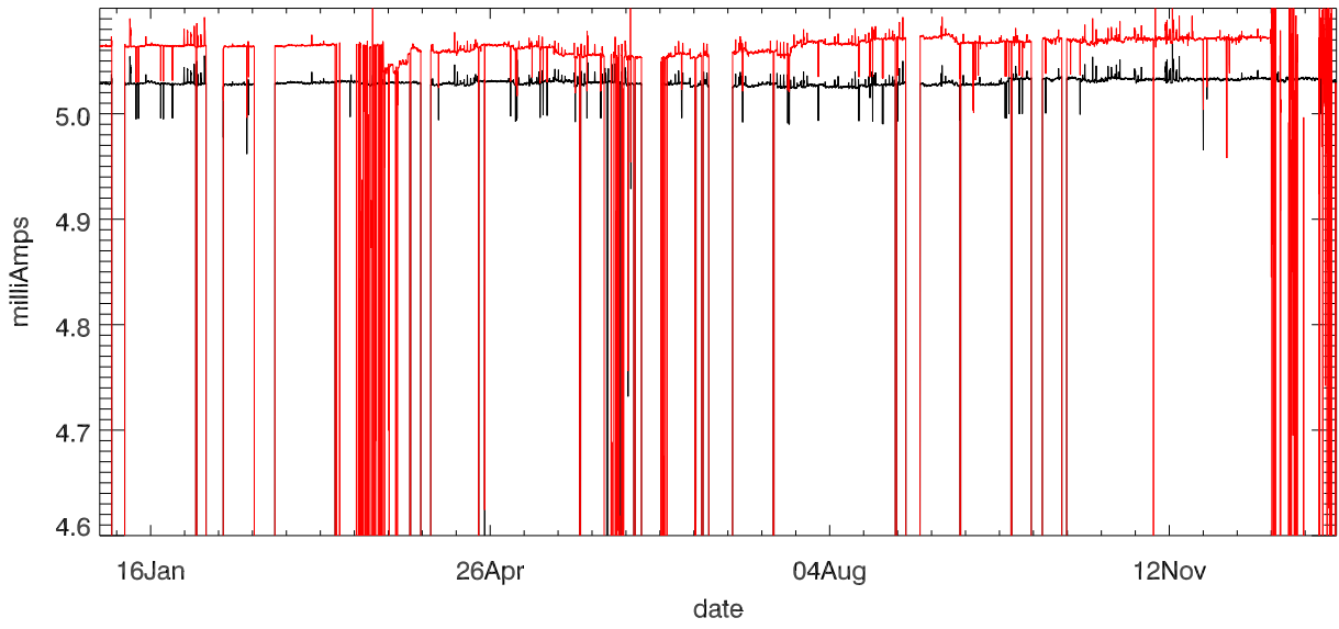
Dewar Current stage 1 (year 2019)
