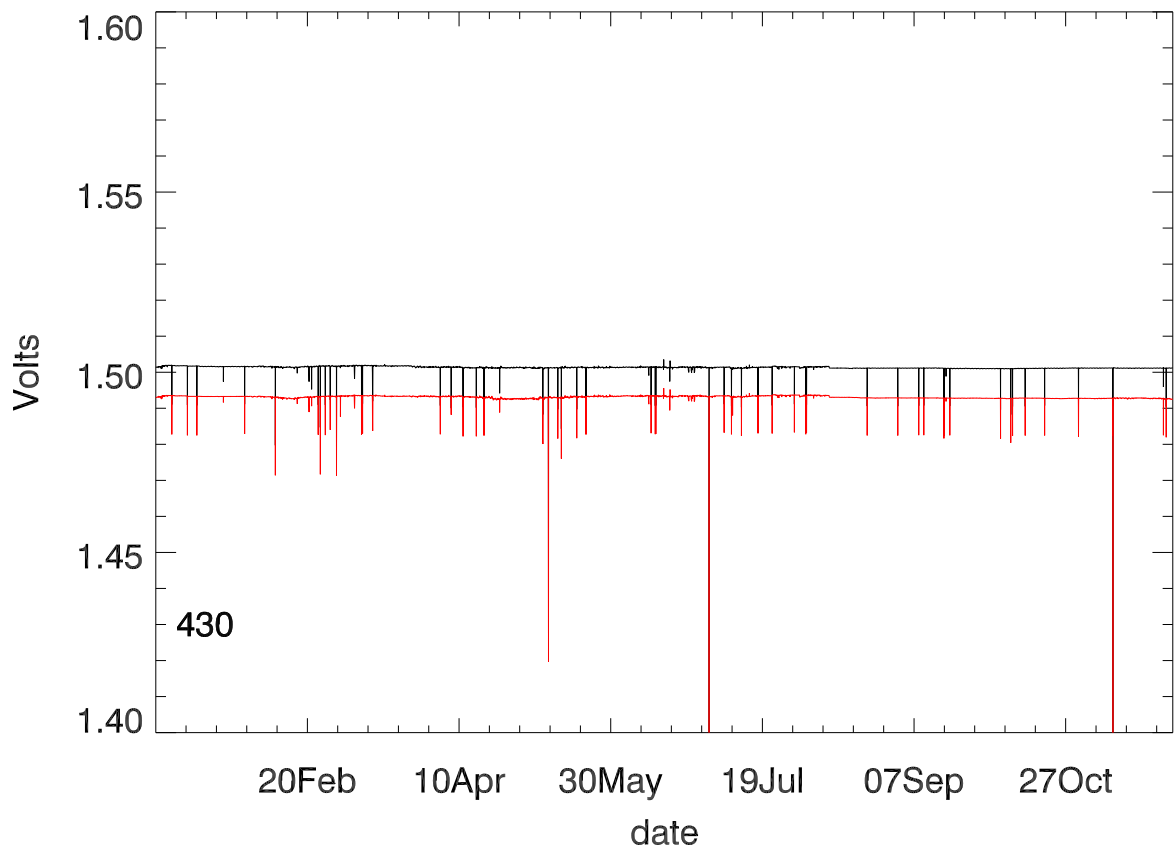
Dewar voltage stage 2 (year 2020)
