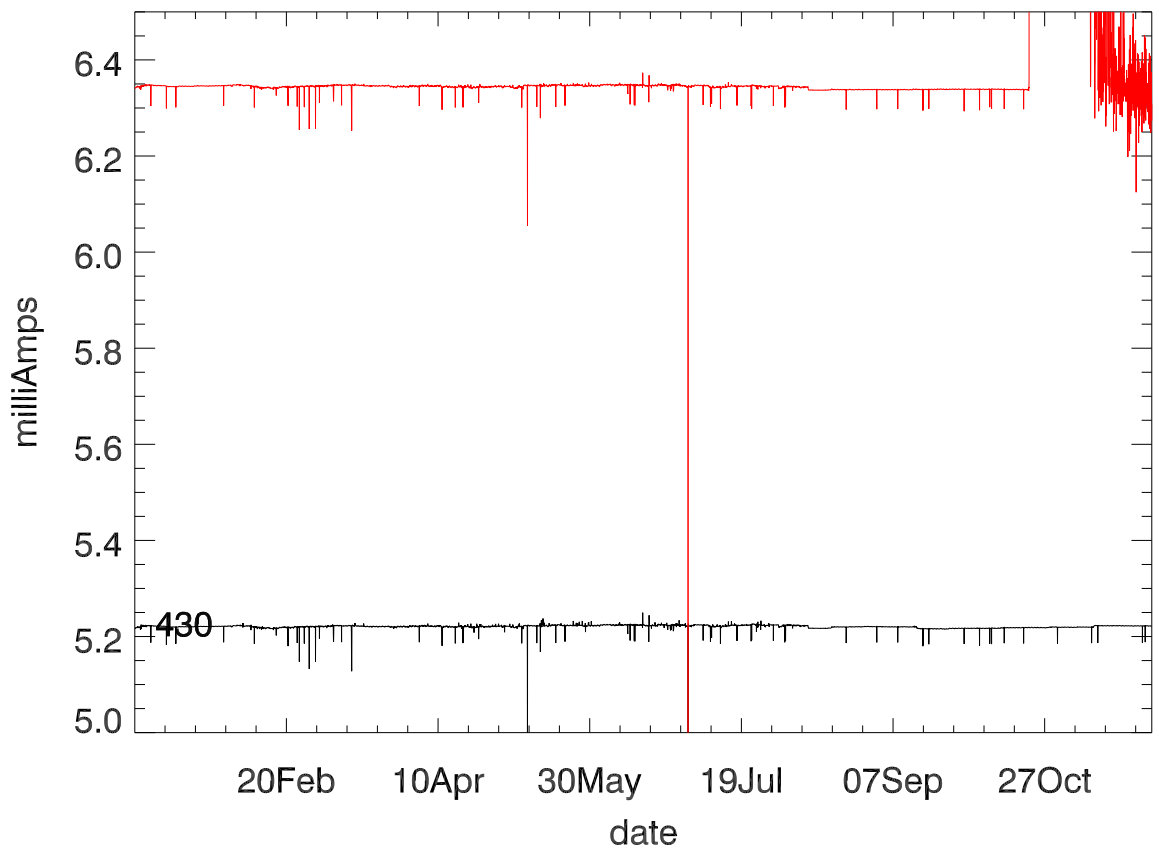
Dewar Current stage 2 (year 2020)
