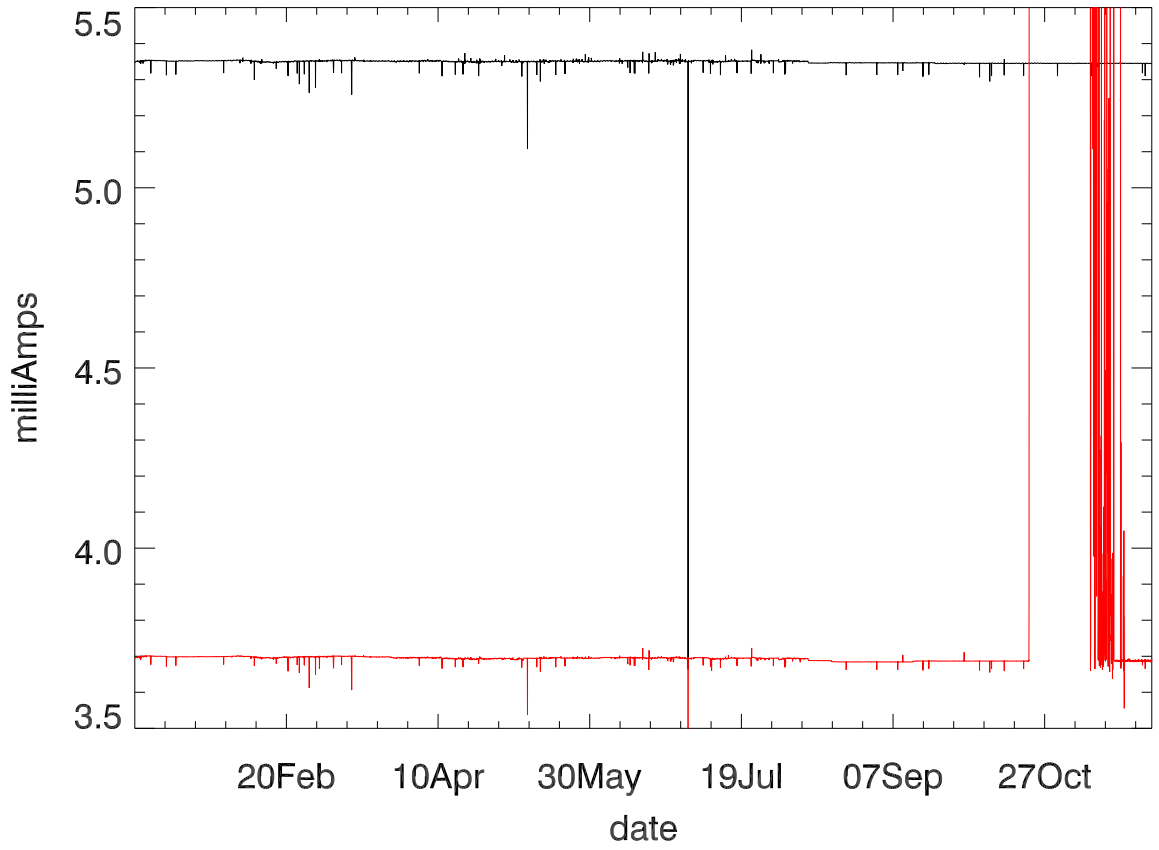
Dewar Current stage 1 (year 2020)
