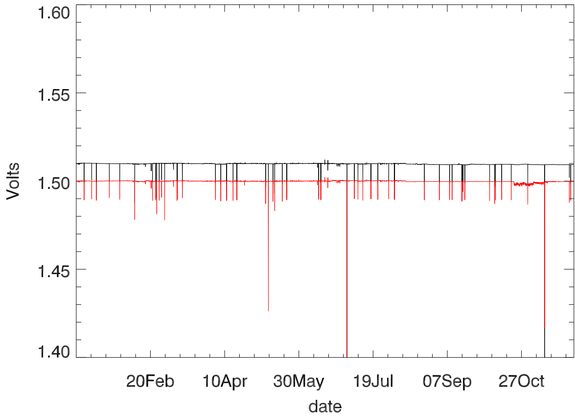
Dewar voltage stage 1 (year 2020)
