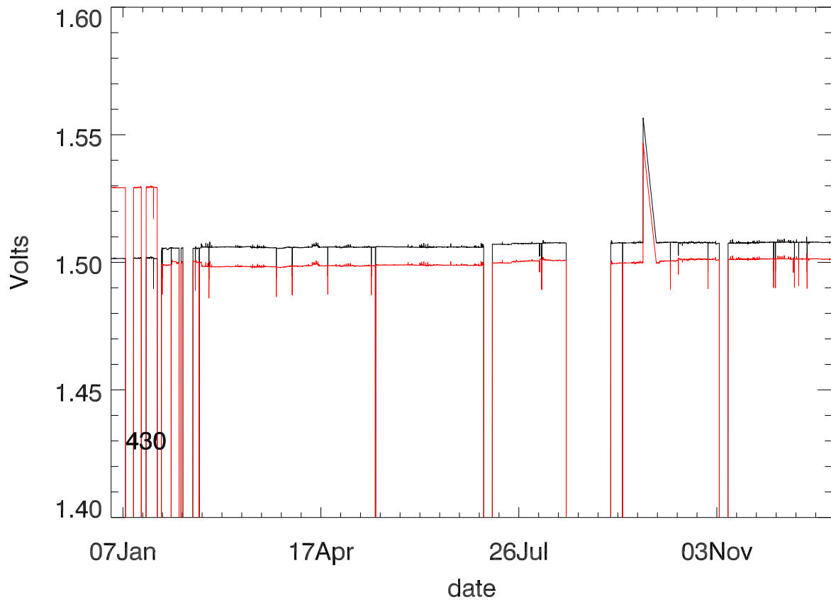
Dewar voltage stage 2 (year 2013)
