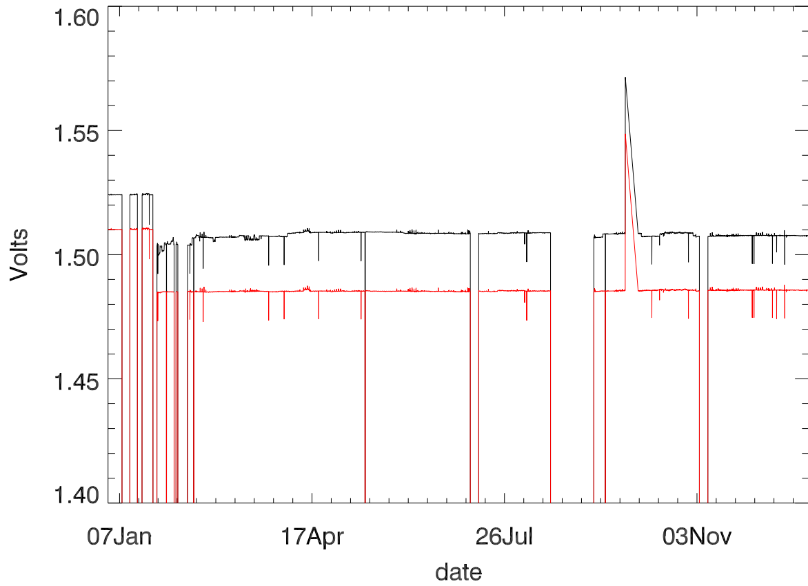
Dewar voltage stage 1 (year 2013)
