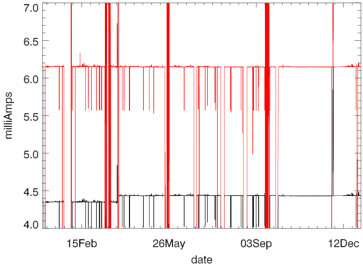
Dewar Current stage 1 (year 2017)
