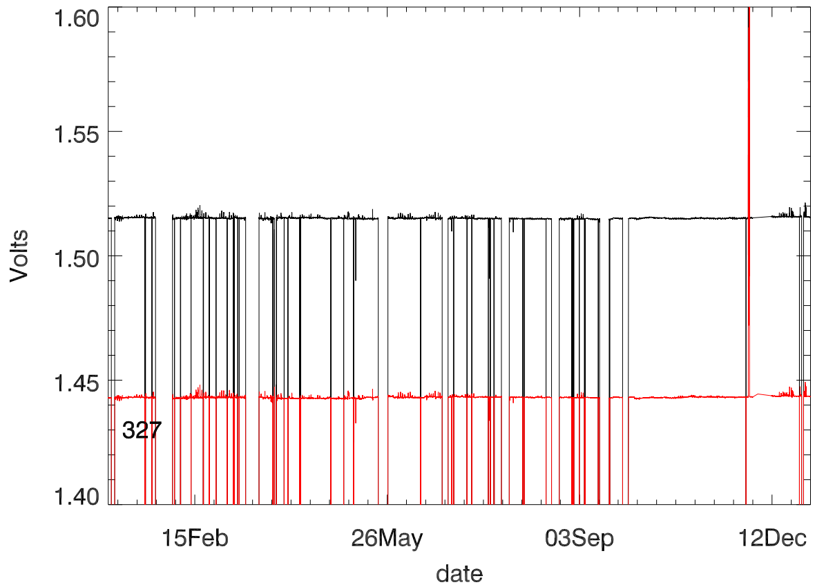
Dewar voltage stage 2 (year 2017)
