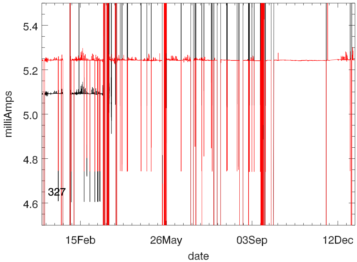
Dewar Current stage 2 (year 2017)
