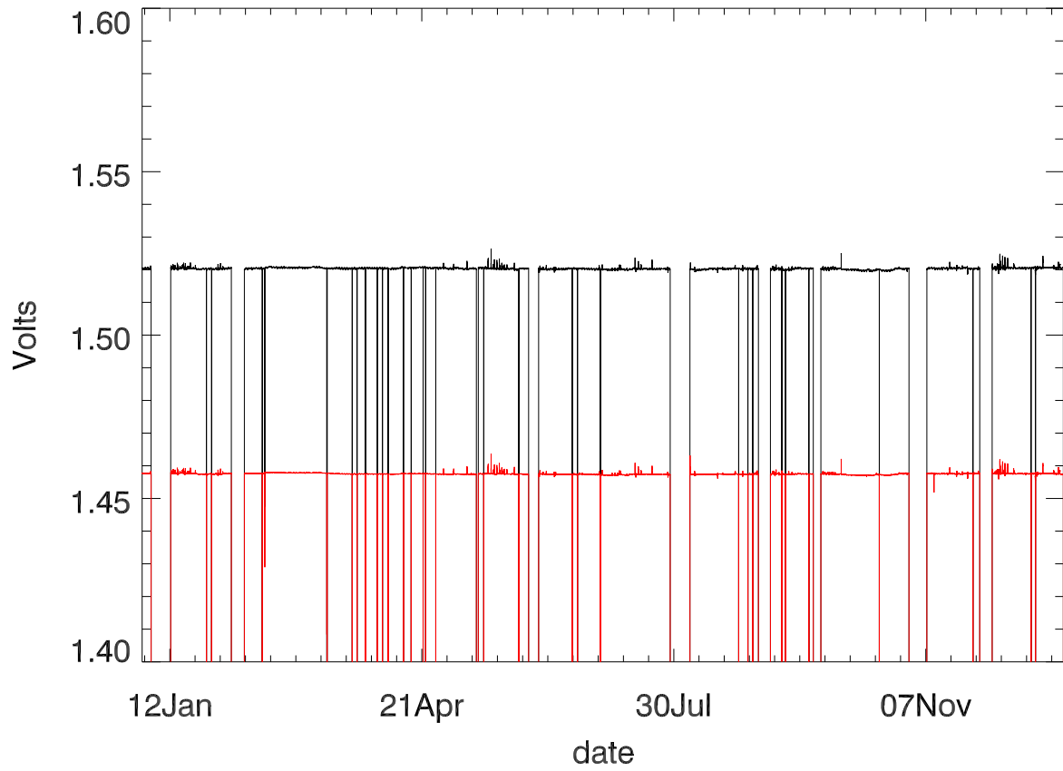
Dewar voltage stage 1 (year 2016)
