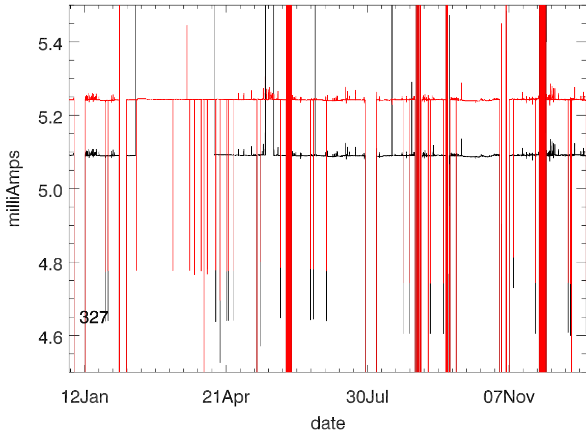
Dewar Current stage 2 (year 2016)
