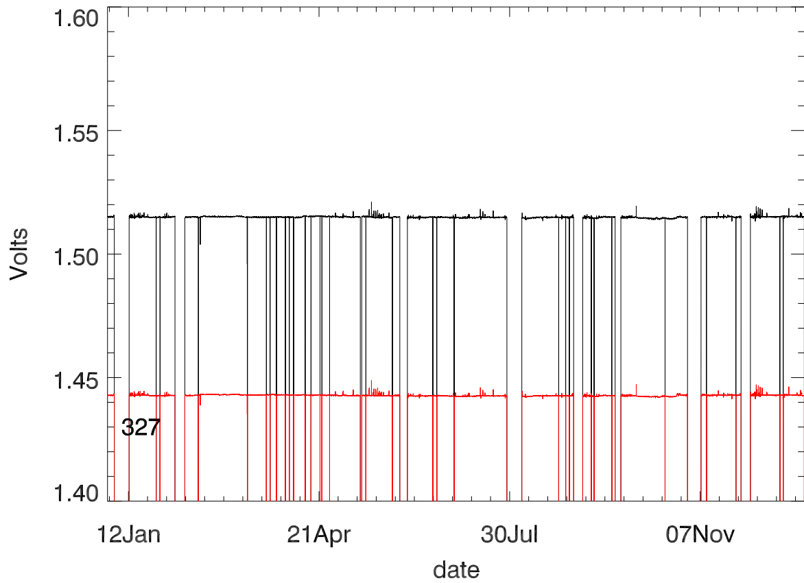
Dewar voltage stage 2 (year 2016)
