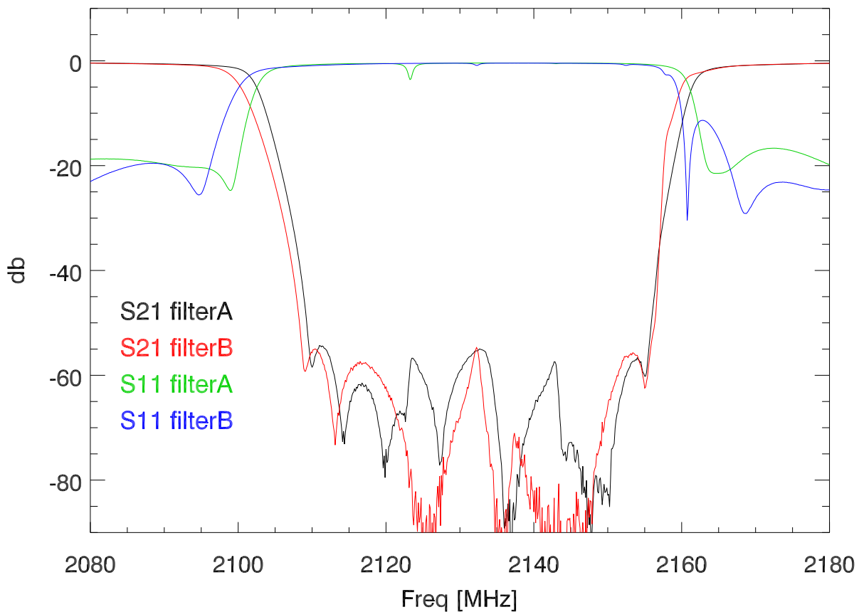
22sep15: SBW notched filters, S21, S11
