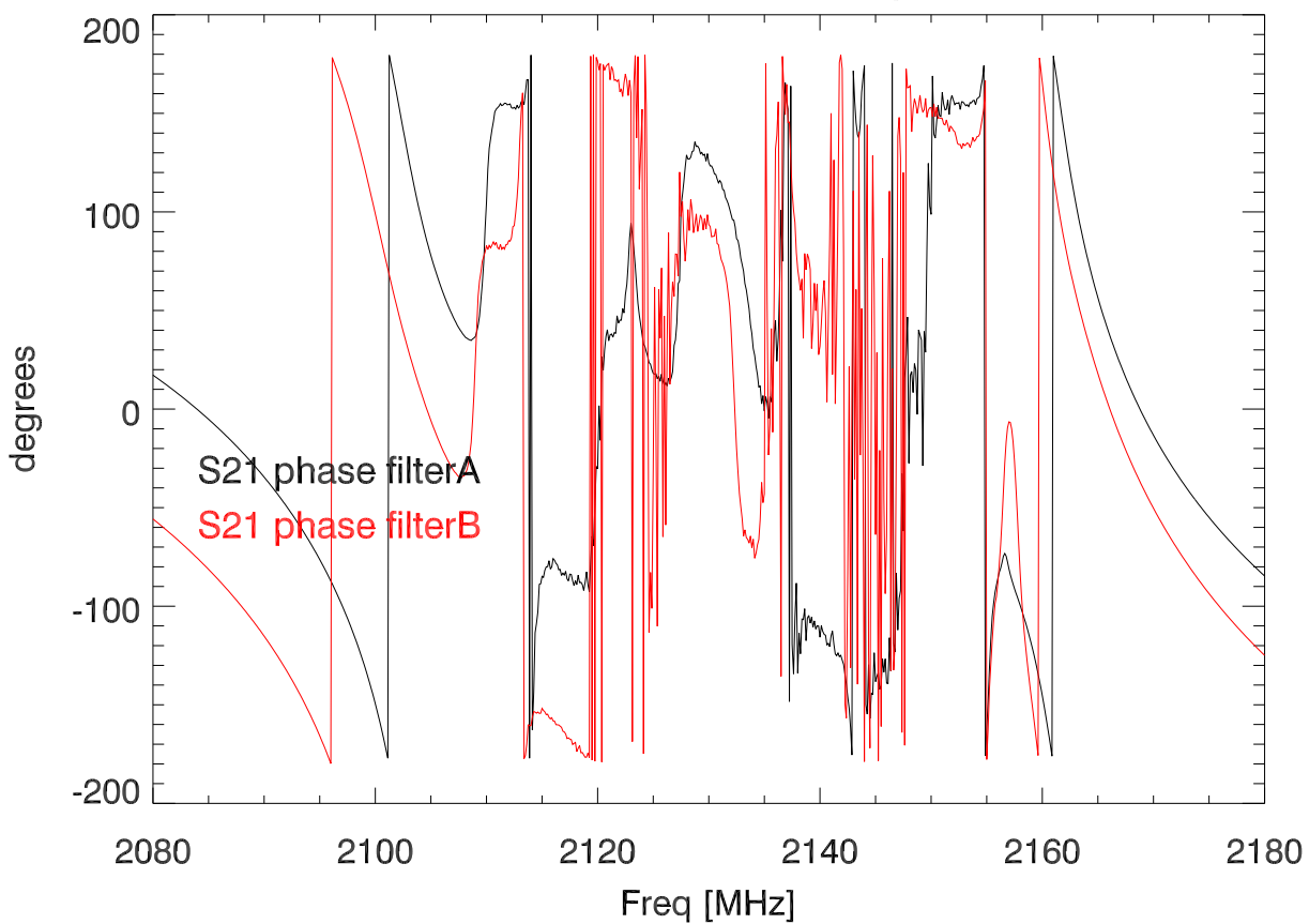
SBW notched filters S21 phase
