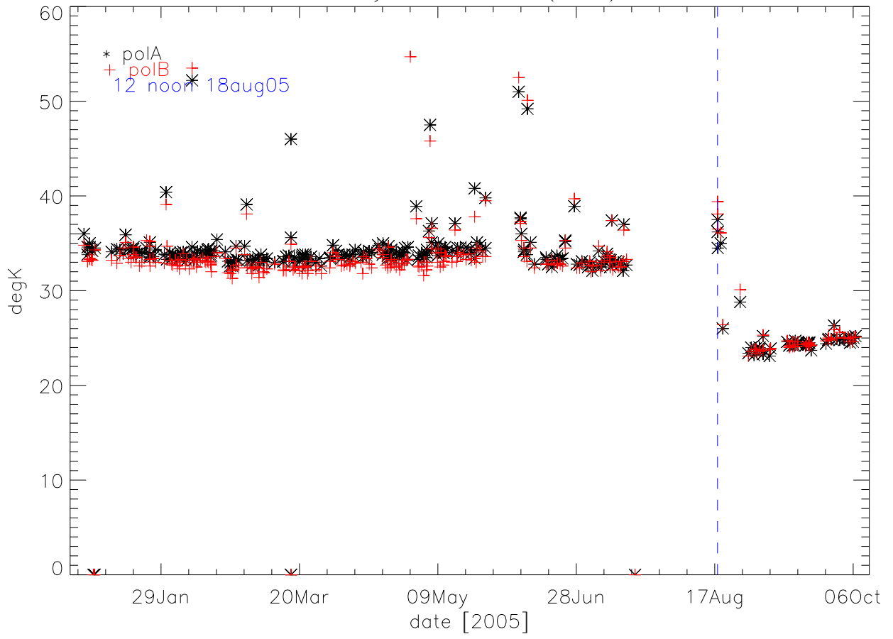
2005 sbw Tsys measured (Hcal) vs date
