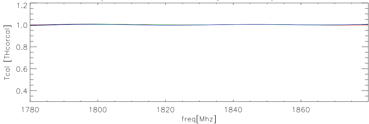
26sep08 OverPlot fits to TCal/Thcorcal polB hxc
