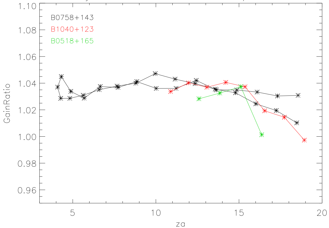
may06 sbTx GainRatio NewHorn/OldHorn
