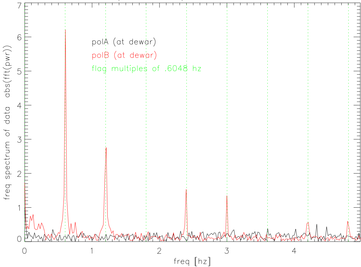
13oct04 sbn spectrum of power data with shutter closed
