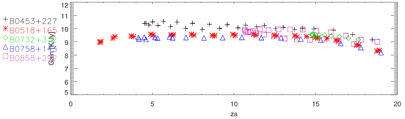
Oct12 Old SbnRcv. Gain K/Jy
