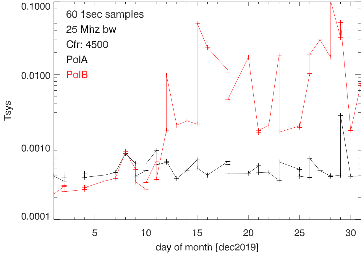
x111 cband rms/mean for cband total power
