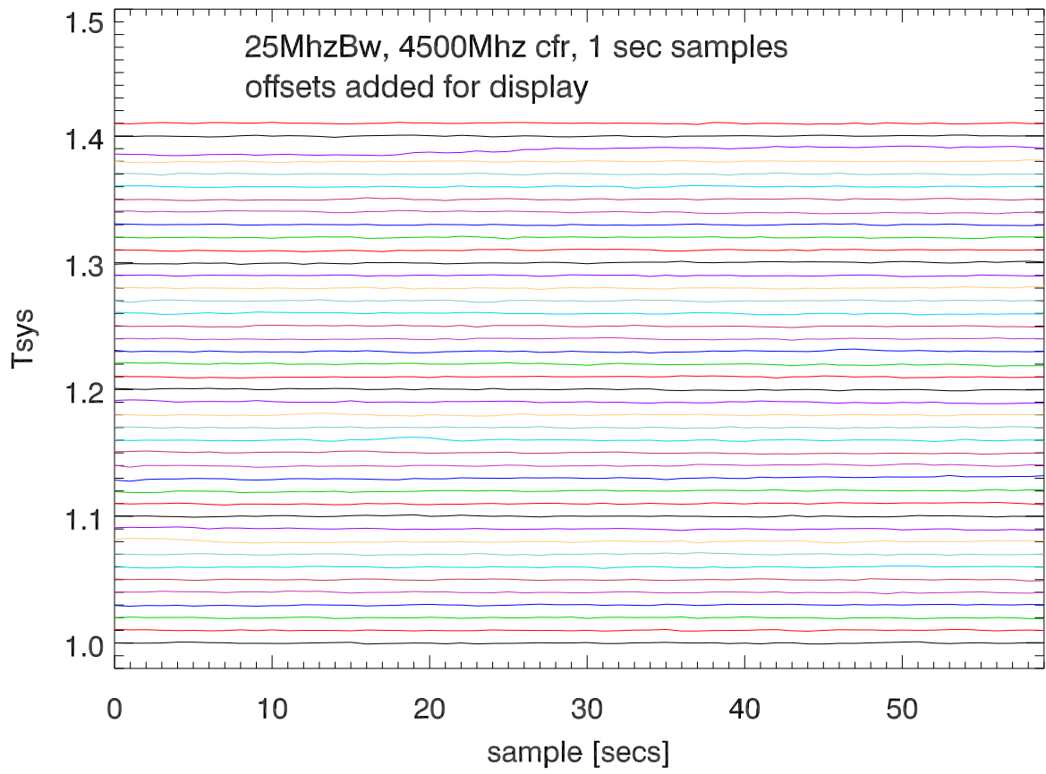
x111 cband totalPwr vs time. Dec2019 (PoIA)
