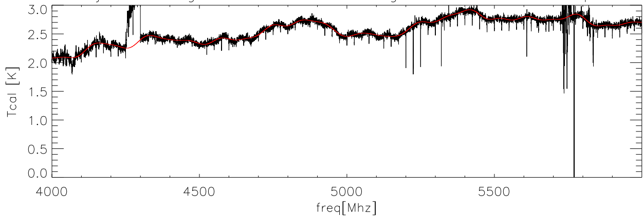
19jul05 Averaged Fits and fit to average for Tcal Kelvins lxcal polA
