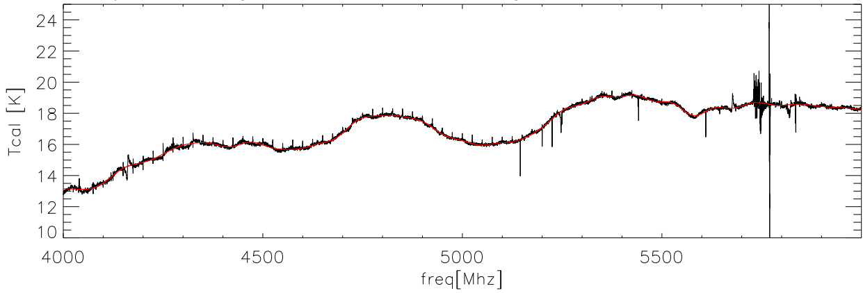
19jul05 Averaged Fits and fit to average for Tcal Kelvins hxcal polB
