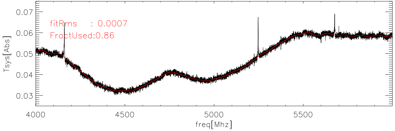
10jun05 Averaged data and fit for CalDeFlection/Tsys on abs polB
