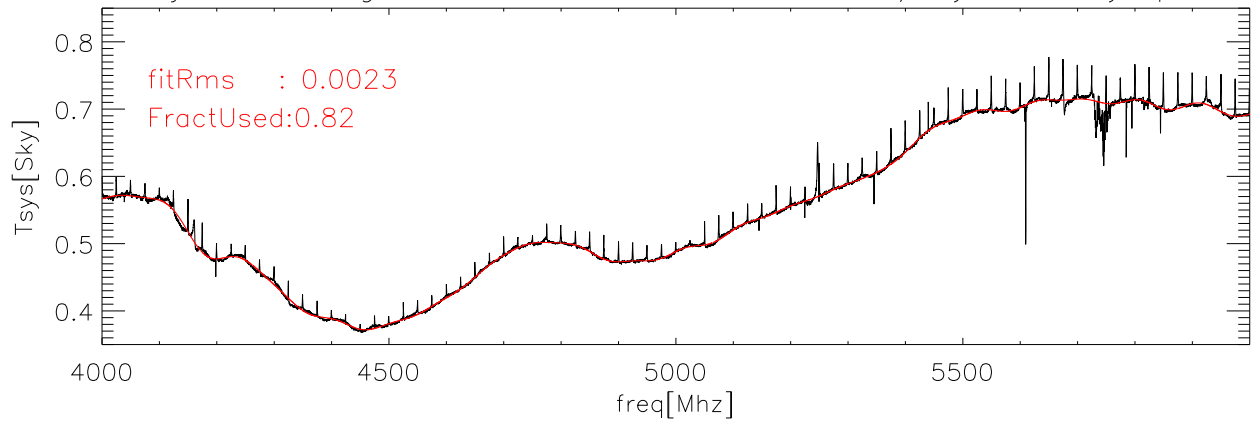
10jun05 Averaged data and fit for CalDeFlection/Tsys on Sky polB
