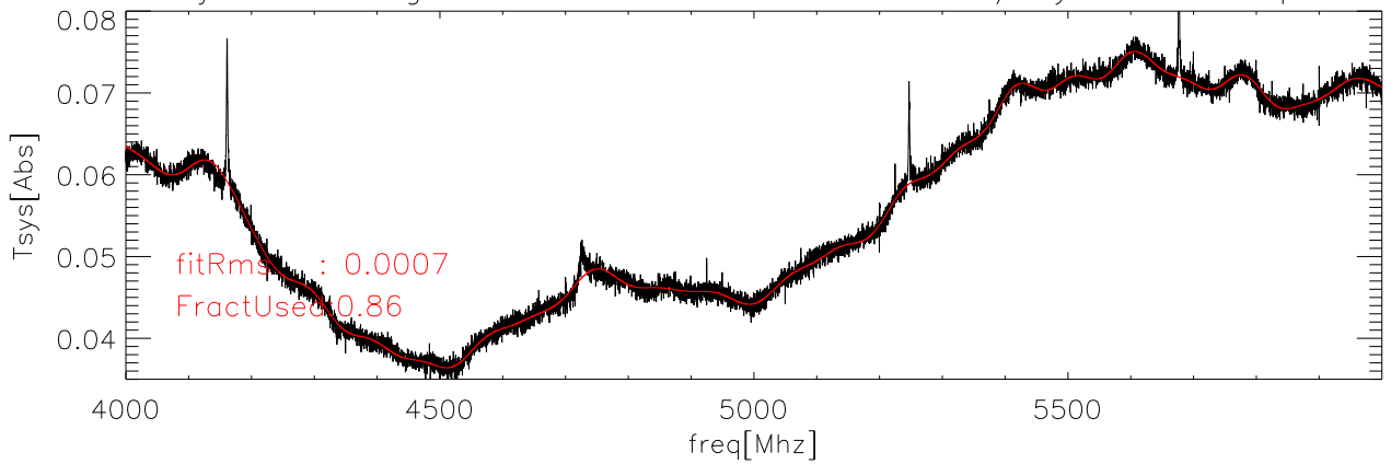
10jun05 Averaged data and fit for CalDeFlection/Tsys on Sky polA
