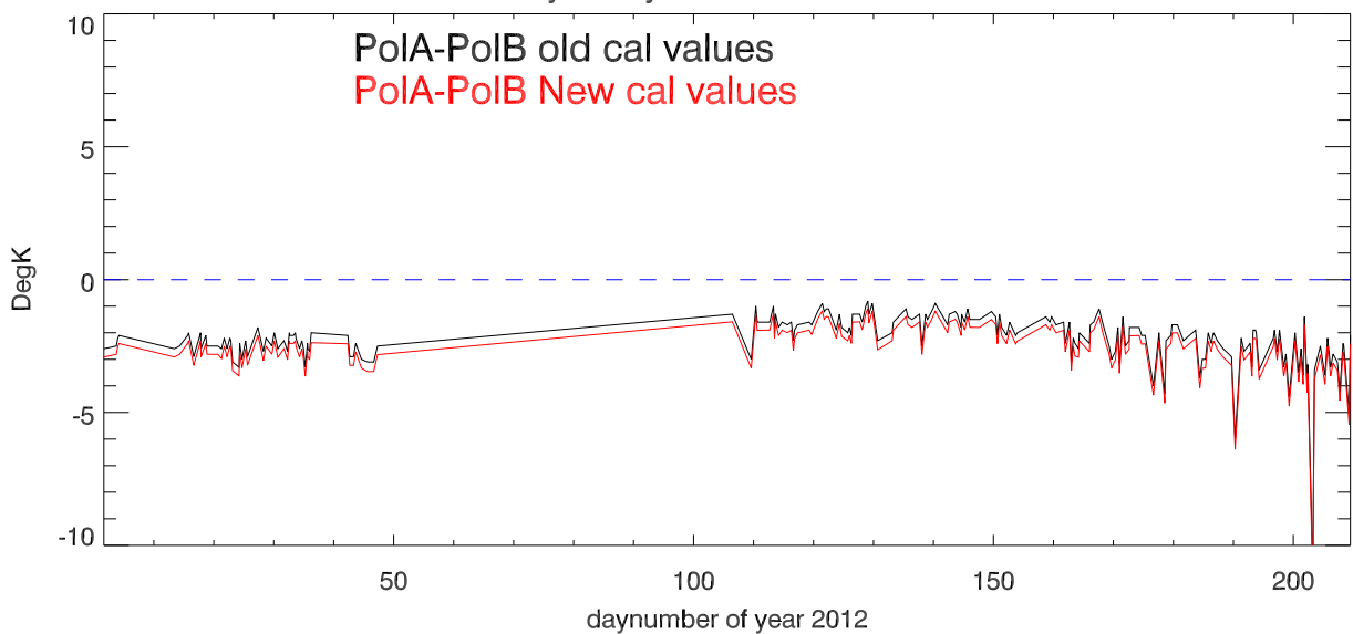
LBW 2012 TsysA-TsysB with old and new calValues
