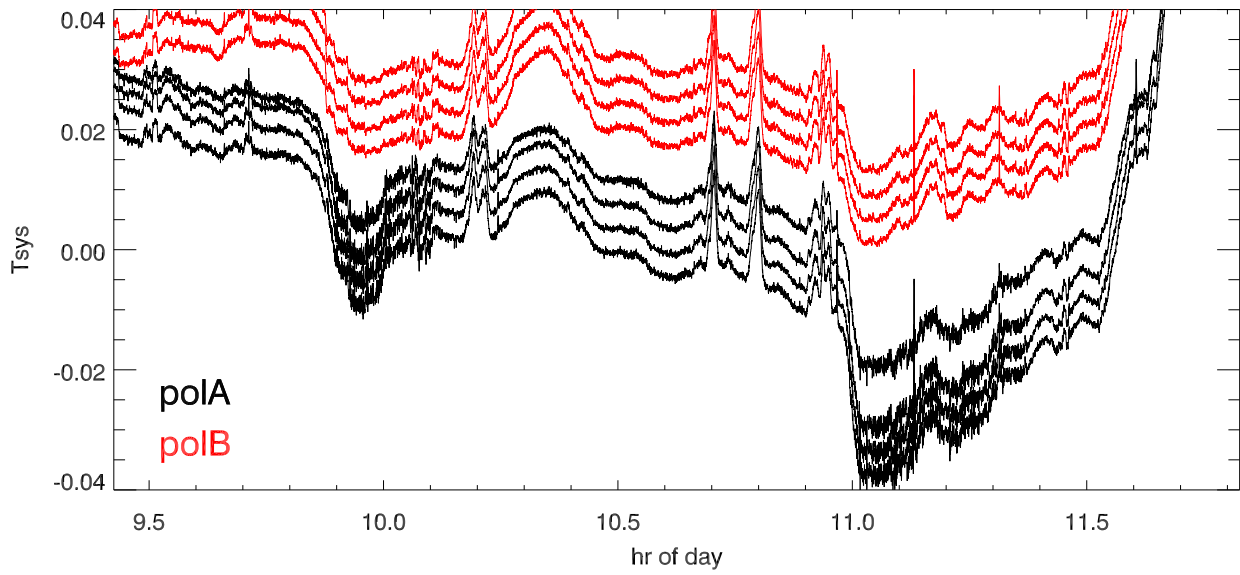
cband Drain voltages
