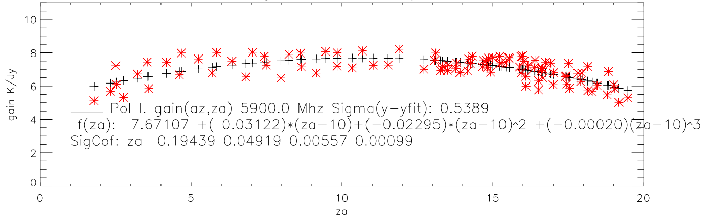
cb 5900 gain vs za and fit may05-oct05
