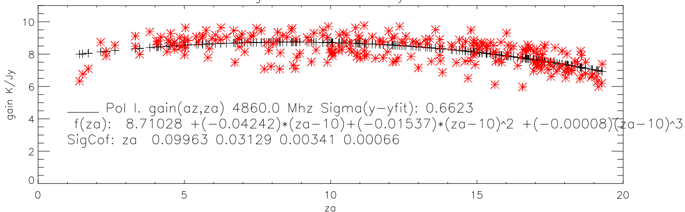
cb 5000 gain vs za and fit may05-oct05
