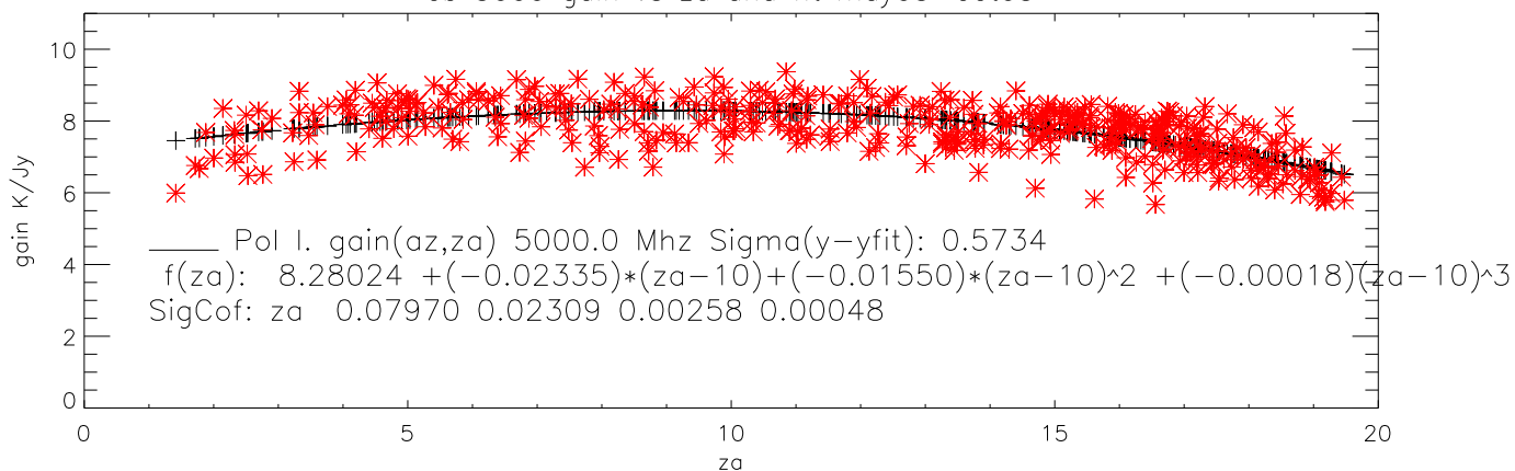
cb 5400 gain vs za and fit may05-oct05
