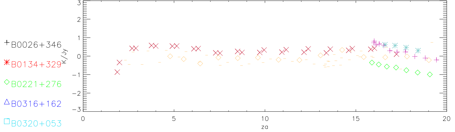
cb 4400 Mhz gain fit residuals
