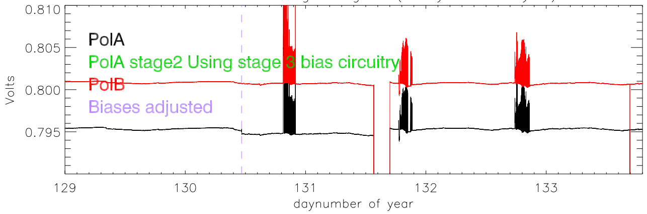
Dewar voltage stage 2,3
