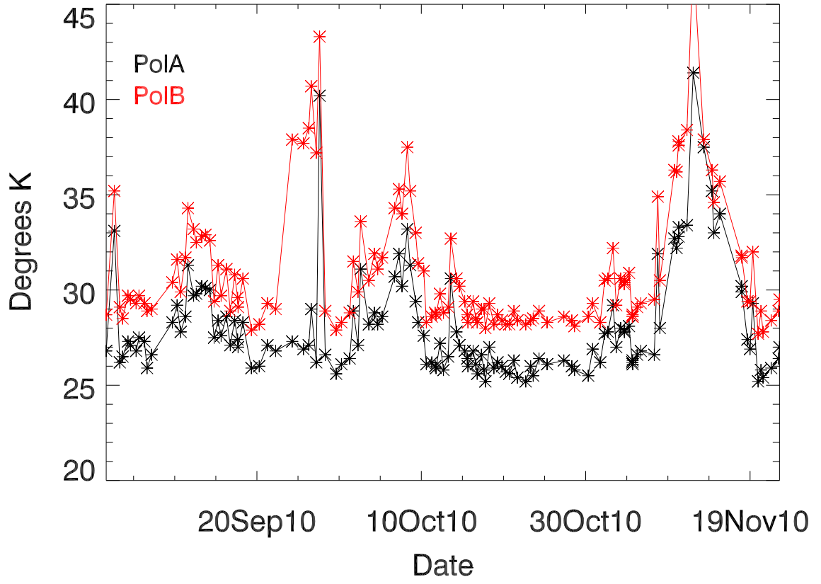
cband 5000 Mhz Tsys vs date
