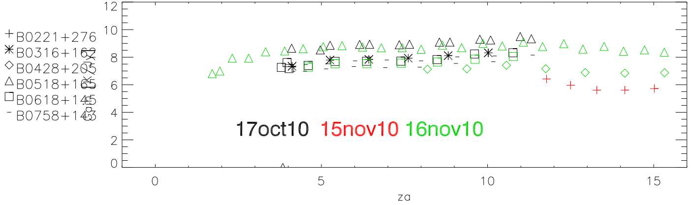
cband calibration runs 17oct,15nov,16nov10: Gain K/Jy
