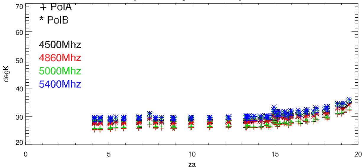
31may12 -> 31aug12 cband. Tsys Vs Za
