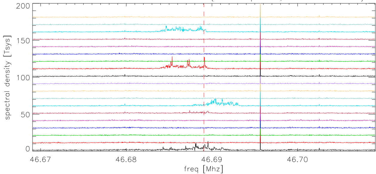
time variable birdie at 46.689Mhz. (1 sec spectra, 31Hz resolution)
