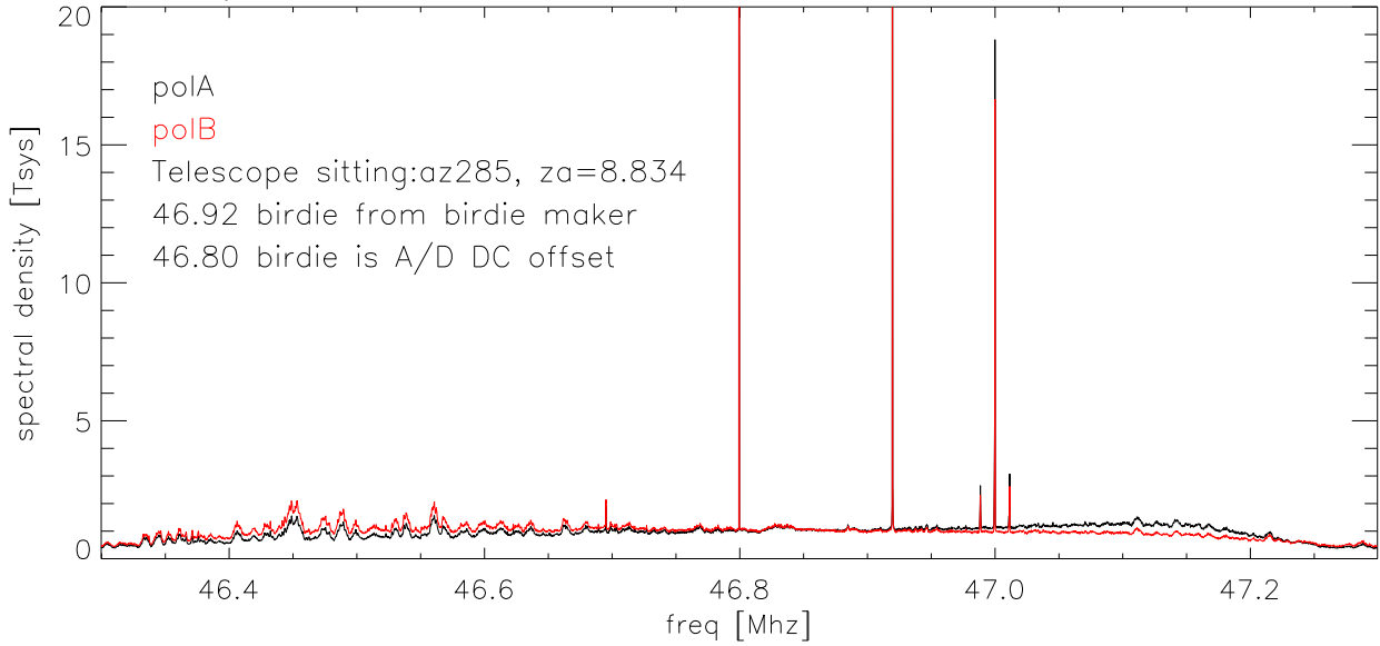
normalized median bandpass blowup vertical scale
