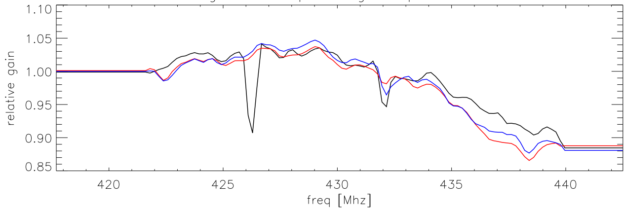
Relative beamWidth vs freq jan05,jul06
