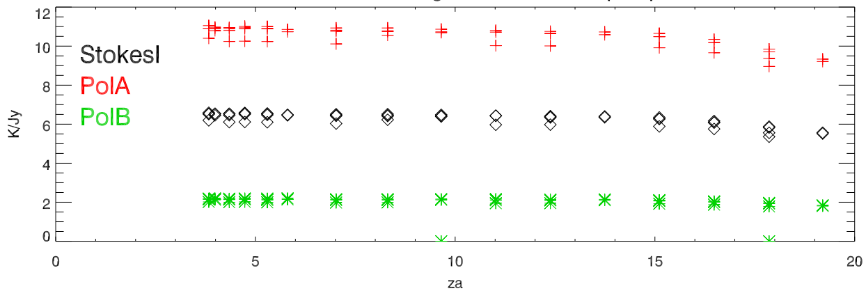
14oct12 B0618+145. 430gr Gain vs za stokesI,polA,polB
