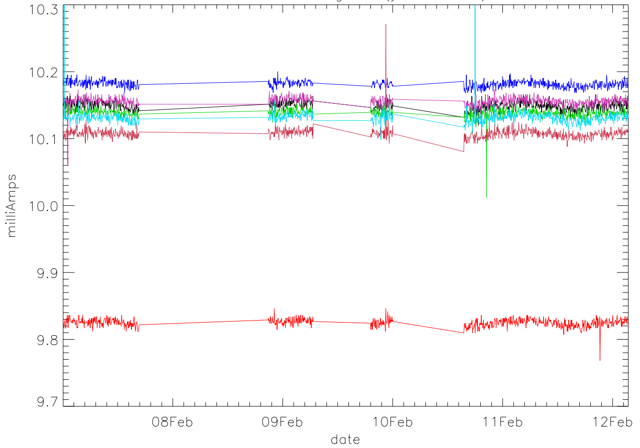
Id:Drain Current. stage 2 (year 2012) PoIB
