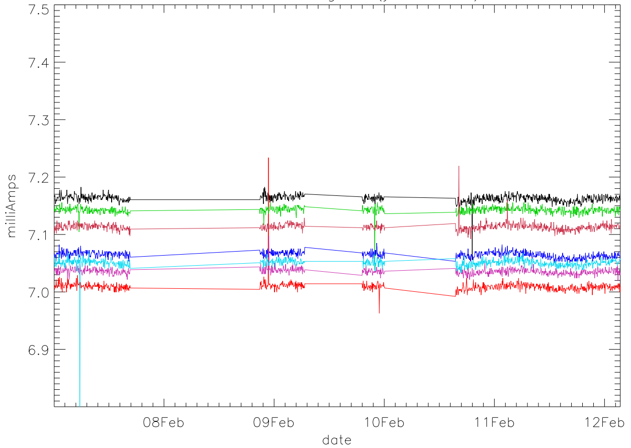
Id:Drain Current. stage 1 (year 2012) PoIB
